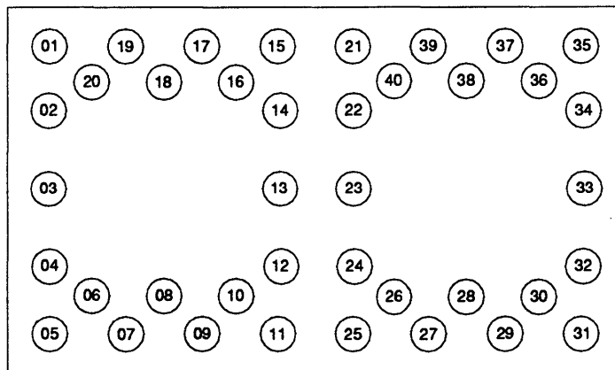
FIGURE 53. SC Die Pinout.
