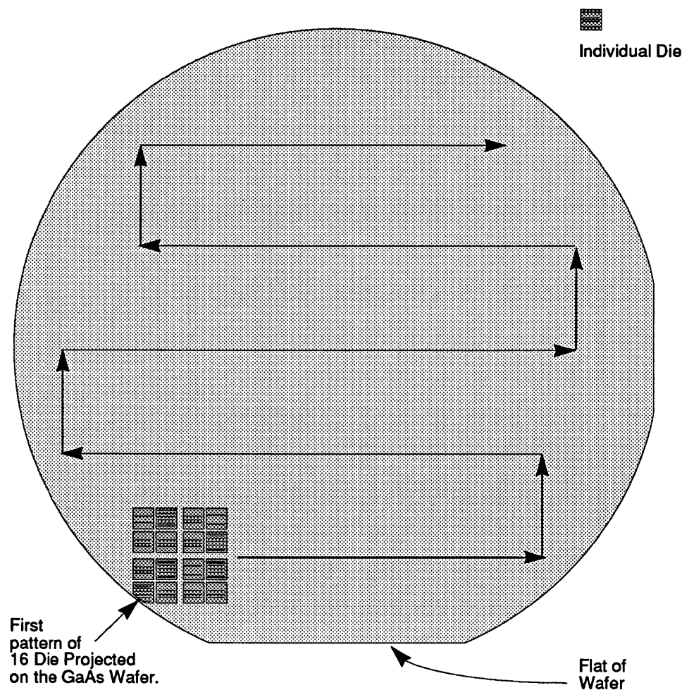
FIGURE 80. Stepping Sequence on a GaAs Wafer.
