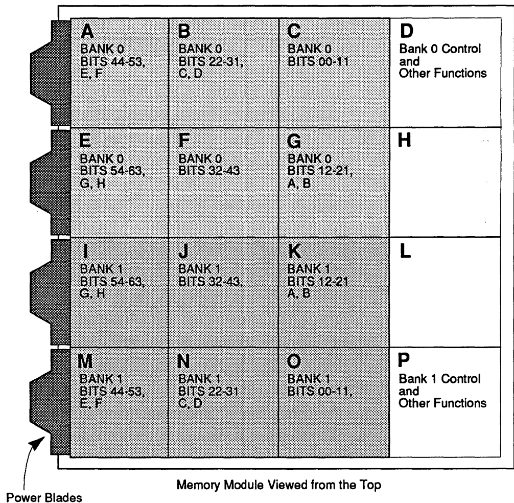
FIGURE 11. Common Memory Stack Usage.
