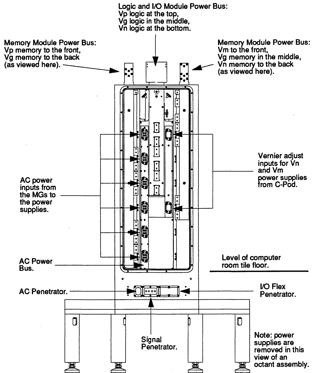
FIGURE 140. Power Distribution in an Octant Assembly.
