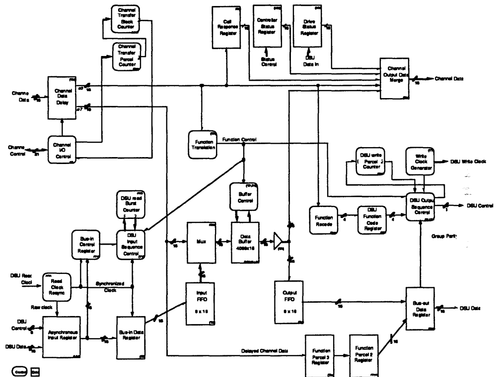
FIGURE 166. Block Diagram of the DD-49/DS-40 Disk Controller.
