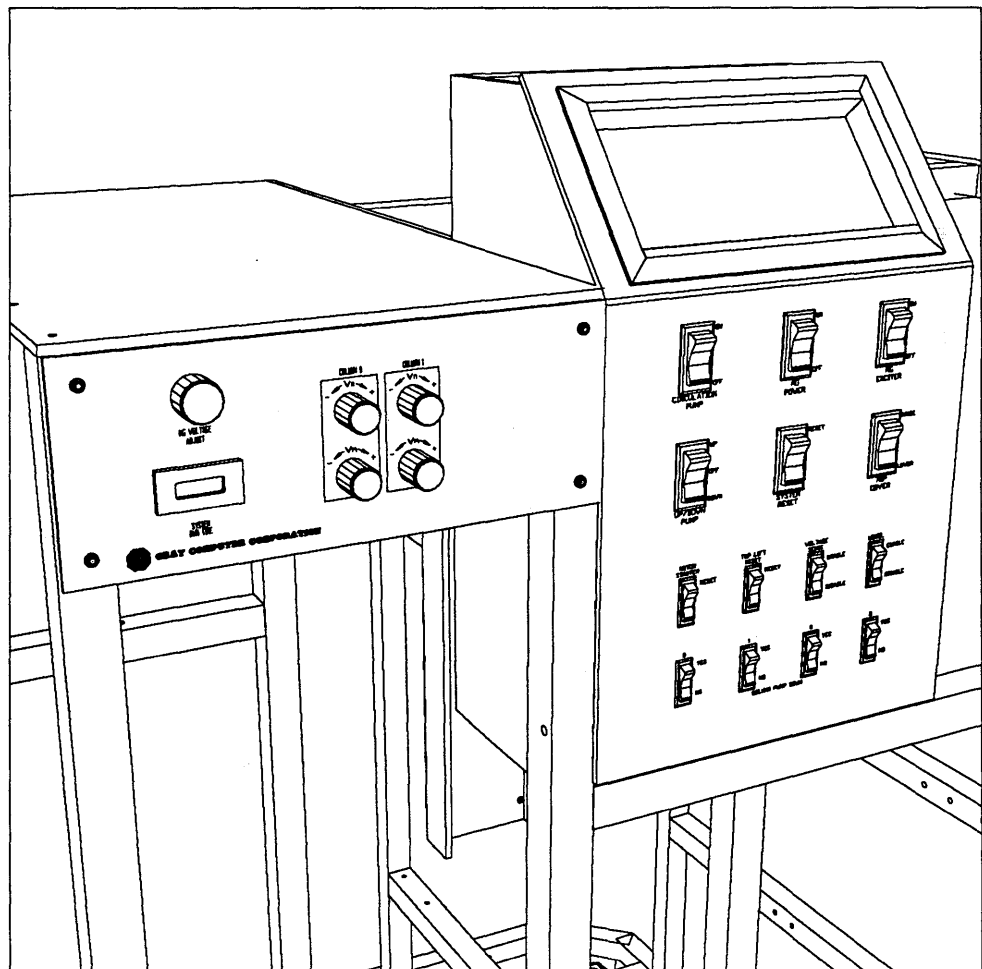
FIGURE 159. Positioning of User Controls and Maintenance Panel.
