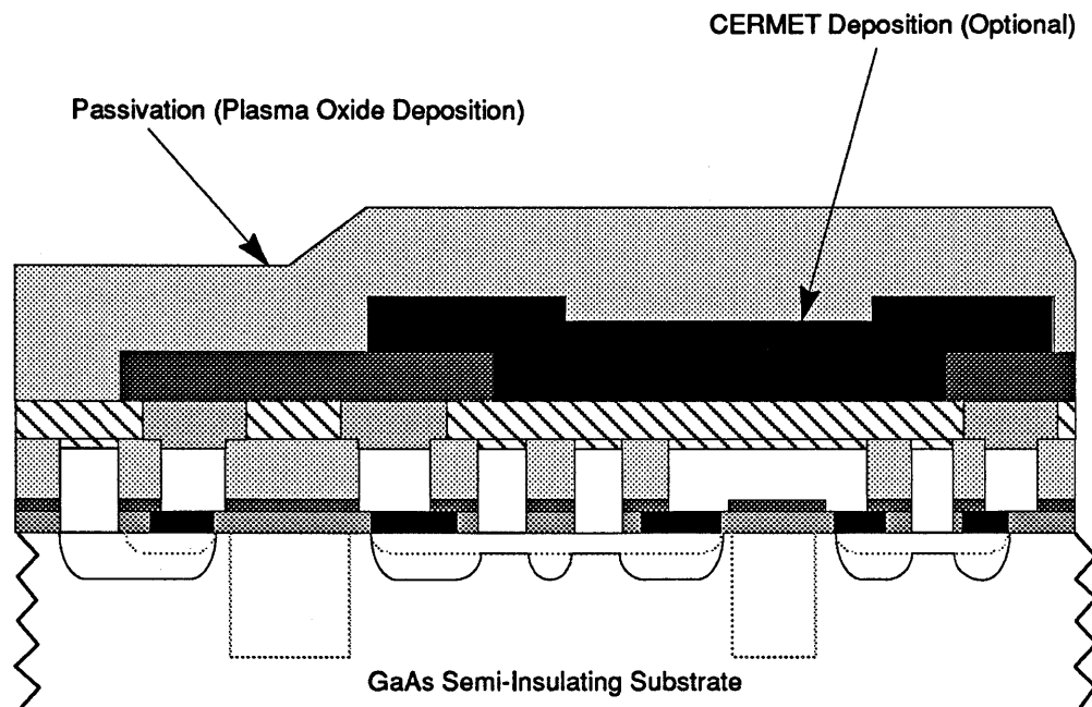
FIGURE 87. CERMET (Optional) and Passivation.
