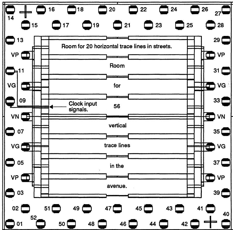
FIGURE 37. Logic Package Pinout.
