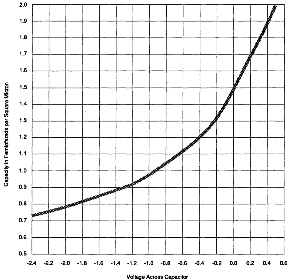
FIGURE 32. Capacitor Electrical Characteristics.
