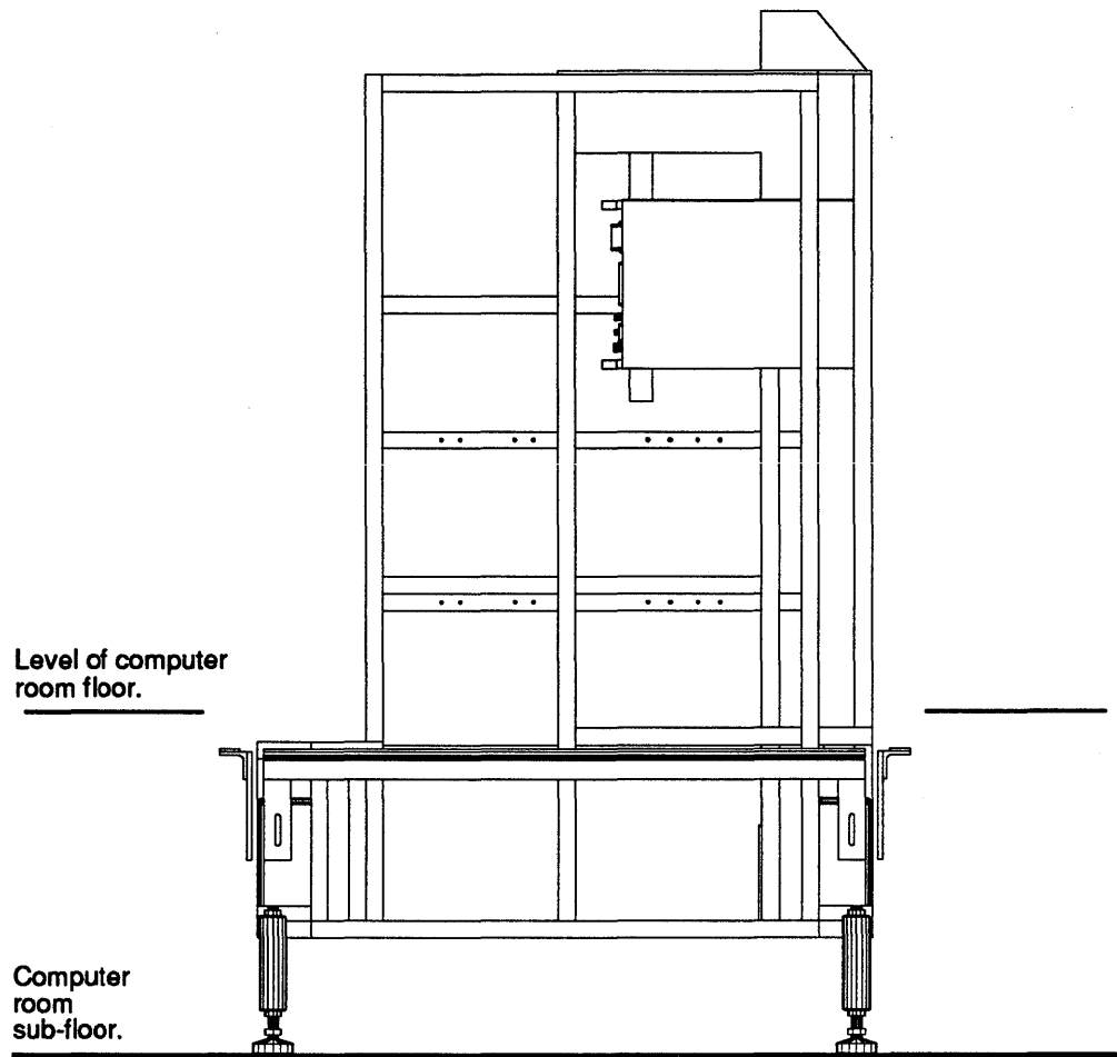
FIGURE 165. Sub-Floor Mounting of the C-Pod.
