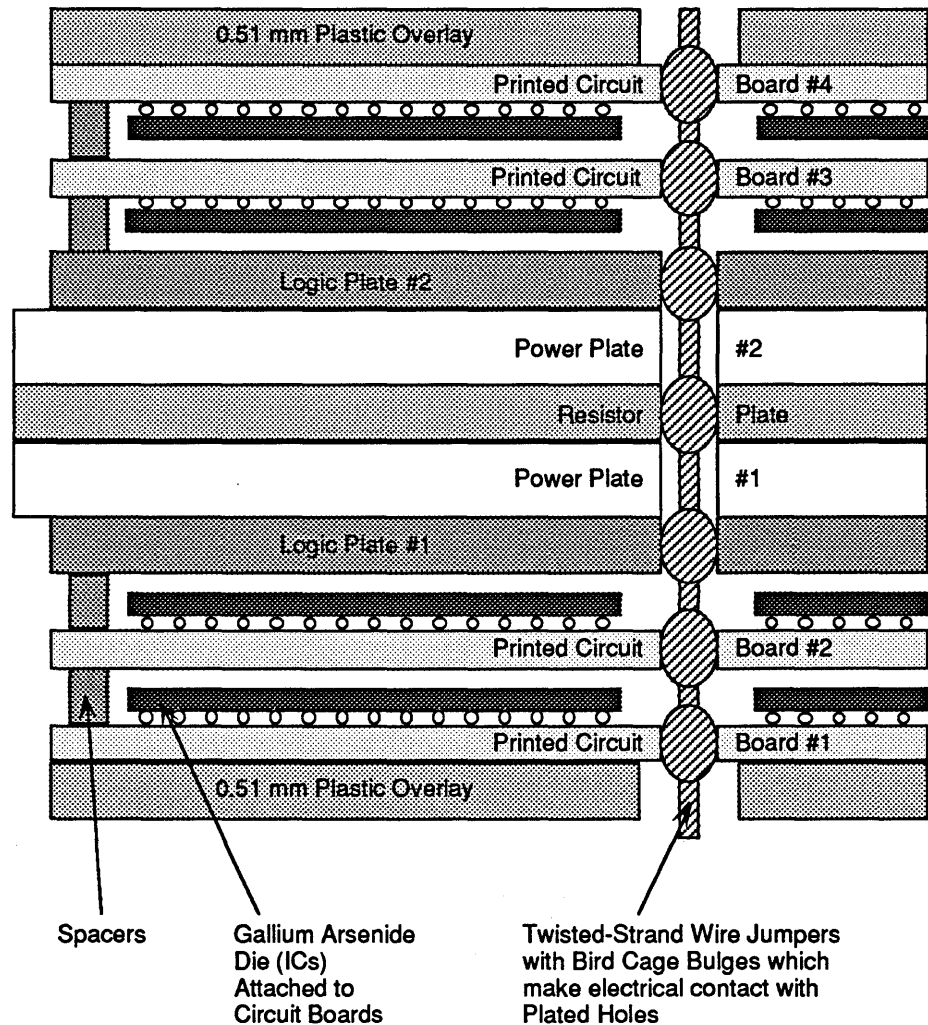
FIGURE 93. Cross Sectional Diagram of a Module.
