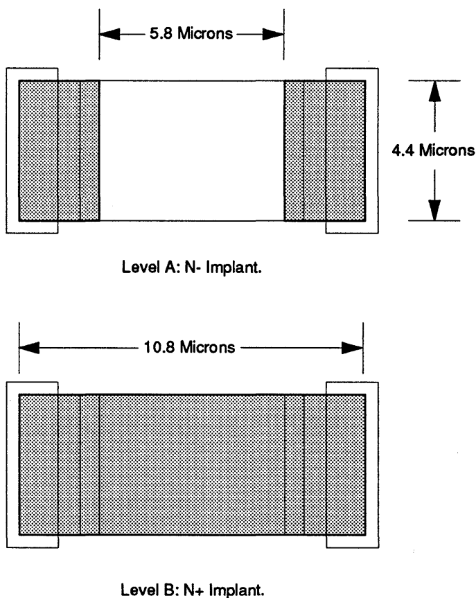
FIGURE 33. Design of a 700 Ohm Resistor—N- and N+ Implants.
