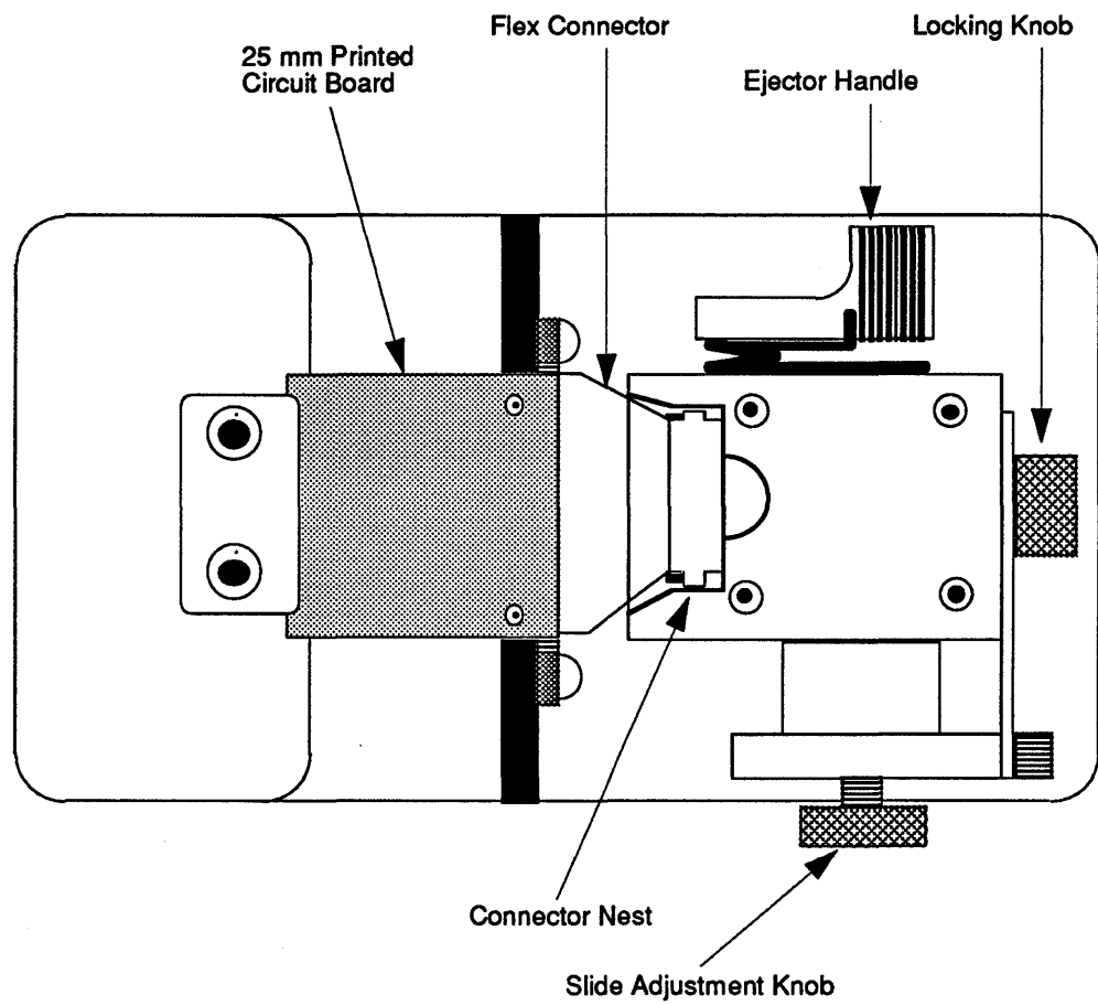
FIGURE 117. Flex Connector Re-Flow Fixture.
