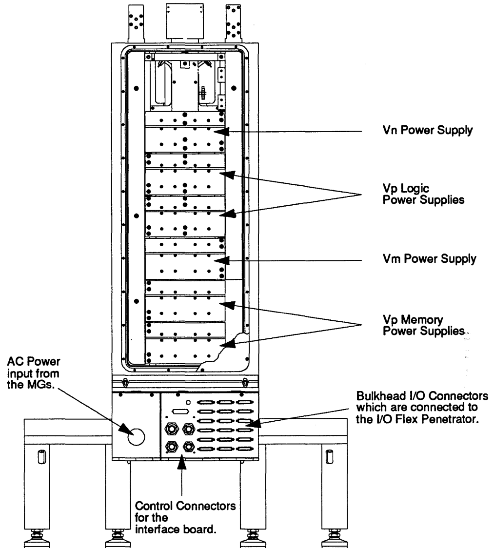
FIGURE 145. Linear Power Supplies In an Octant Assembly.
