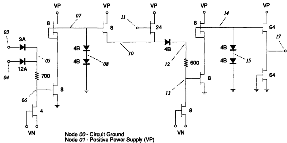
FIGURE 38. DD Cell Schematic Diagram.
