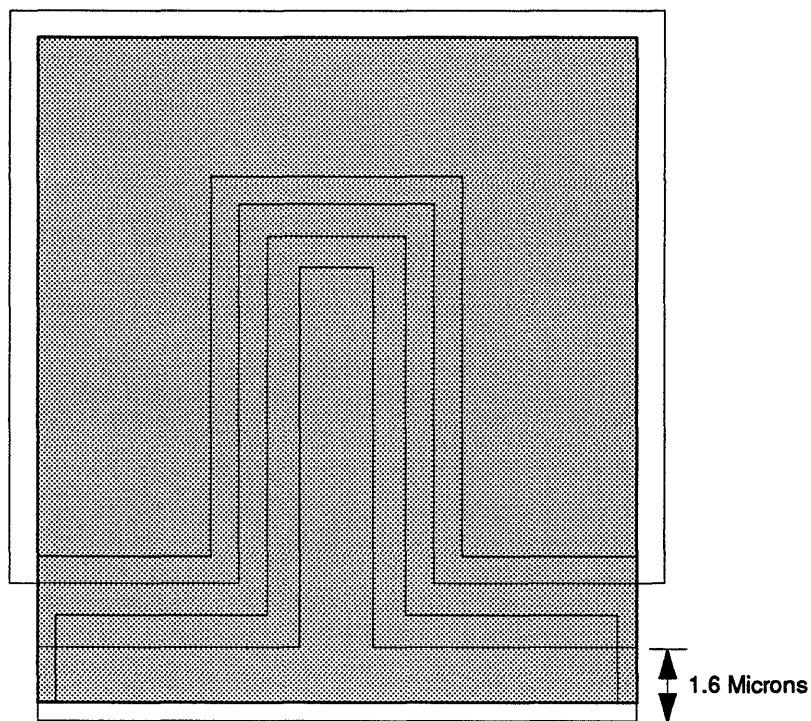
FIGURE 27. Design of a 95 Square Type C Diode/Capacitor.
