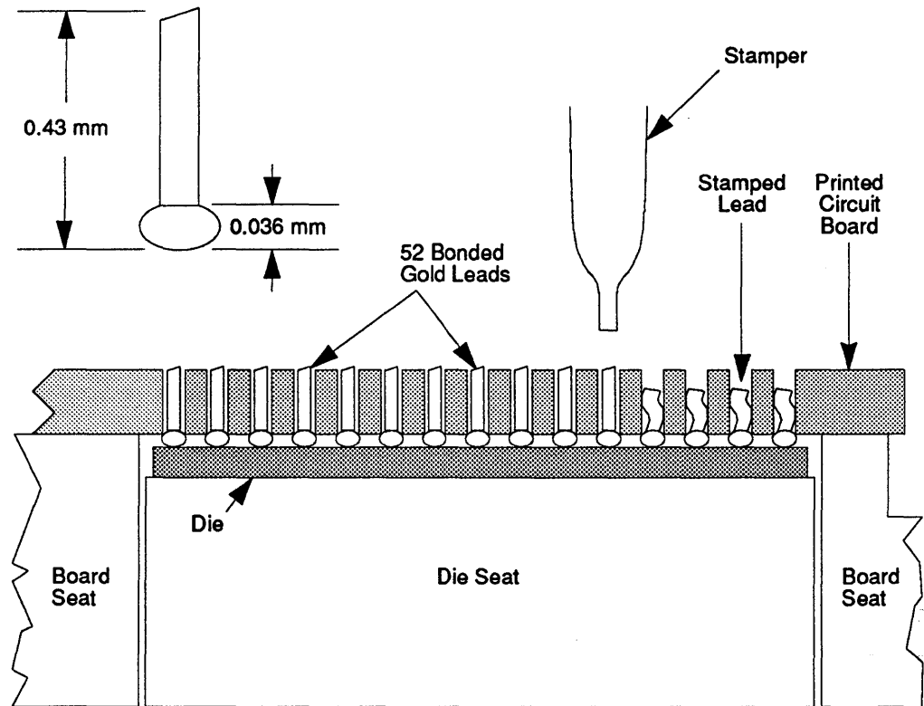
FIGURE 119. Die Attach Stamping Fixture.
