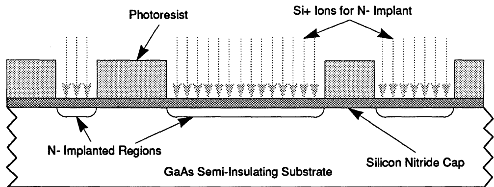
FIGURE 82. Dielectric Encapsulation and N- Implant.
