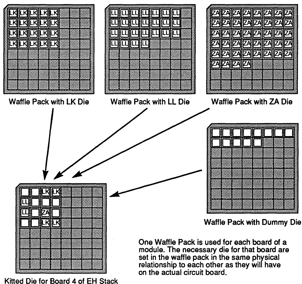
FIGURE 115. The Kitting of Die for a Module.
