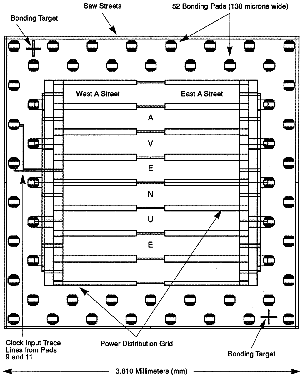
FIGURE 56. Generic IC Assembly.
