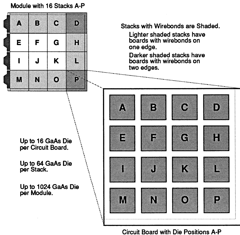
FIGURE 94. Arrangement of Stacks and ICs.
