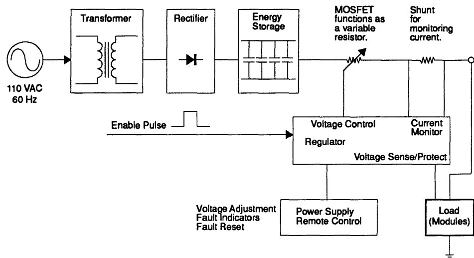
FIGURE 126. Pulse-Power Supply Block Diagram.
