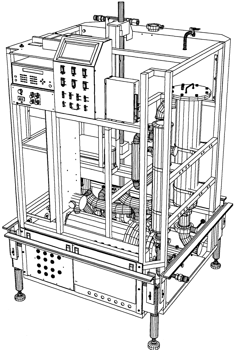
FIGURE 157. C-Pod-Front Right View.
