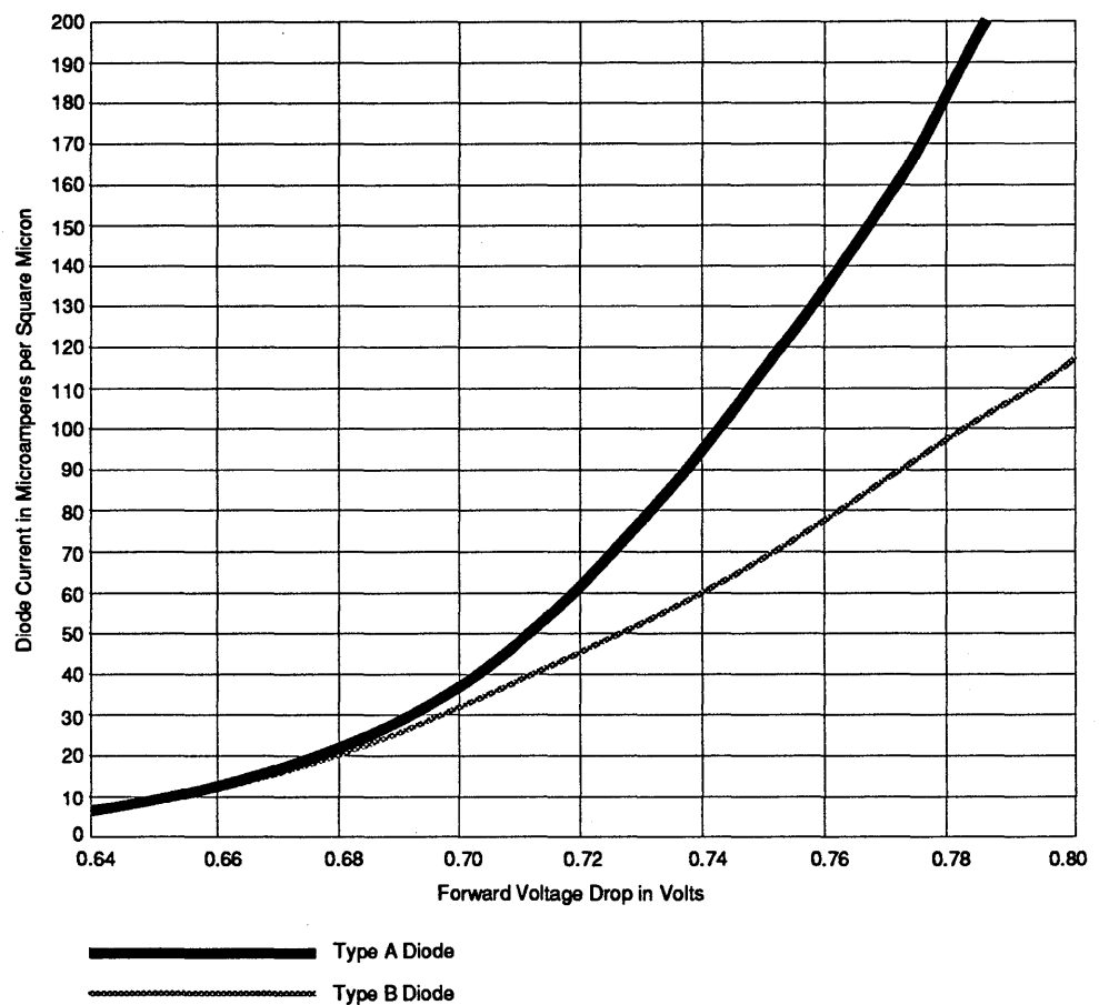
FIGURE 26. Diode Electrical Characteristics.
