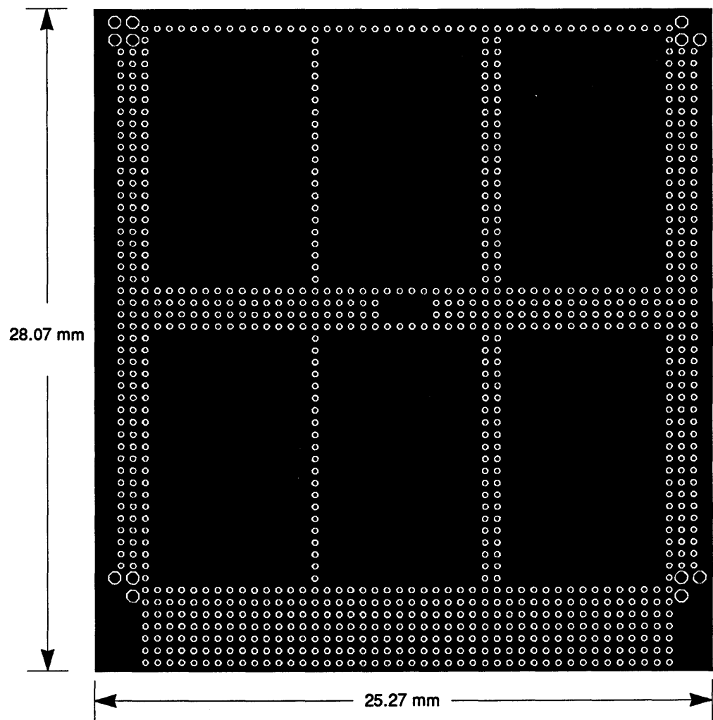
FIGURE 100. One Meg Memory Circuit Board.
