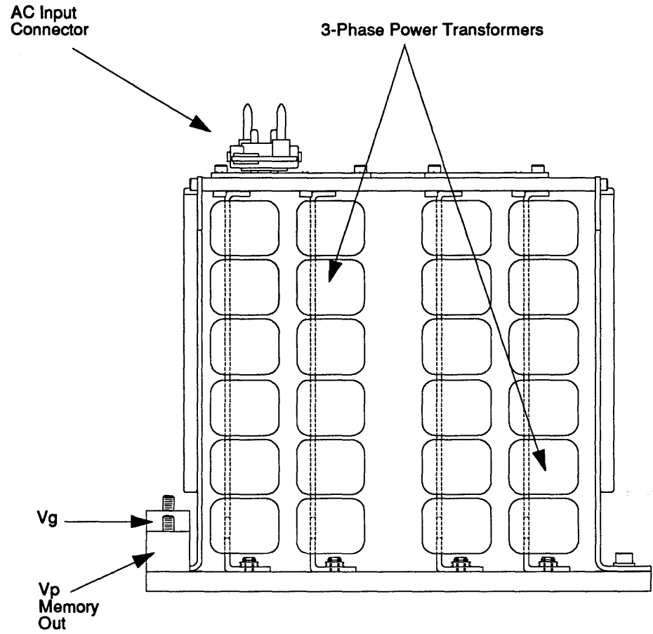
FIGURE 147. Simplified Top View of a Vp Memory Power Supply.
