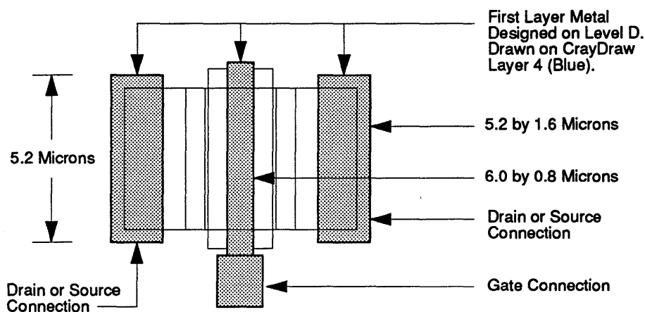
FIGURE 19. 4.0 Micron Transistor—First Layer Metal.
