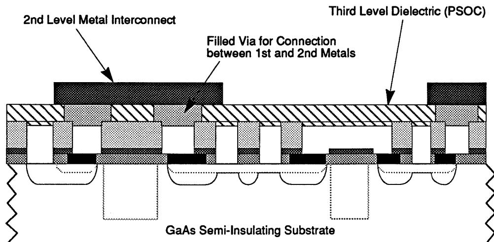
FIGURE 86. Second Level Metal.
