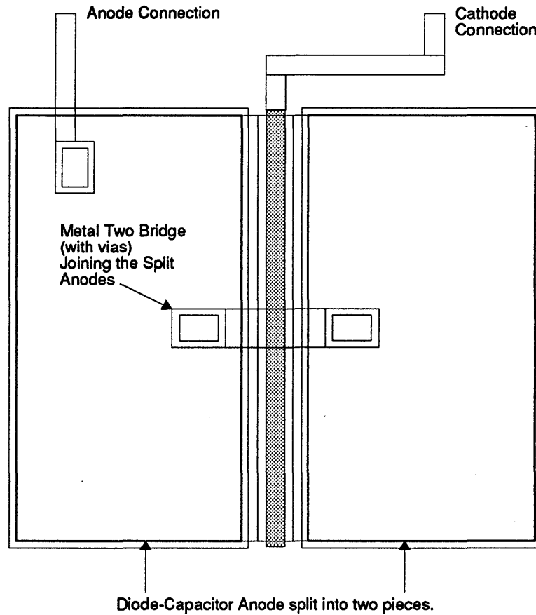
FIGURE 31. Capacitor Broken Into Two Pieces.
