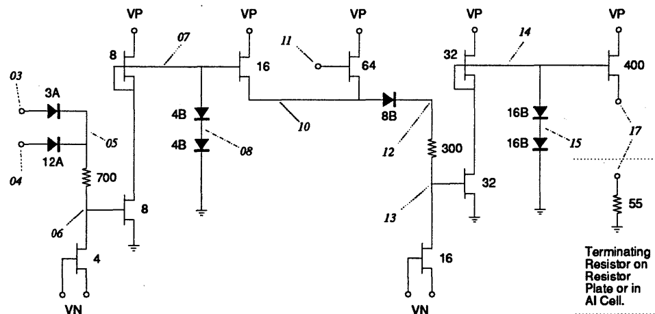
FIGURE 40. FE Cell Circuit Schematic.
