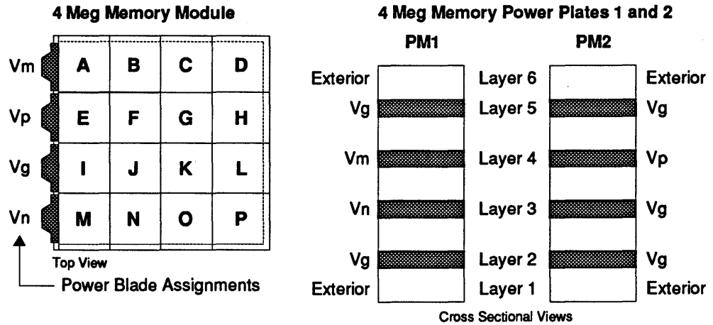
FIGURE 111. Power Distribution in Four Meg Memory Modules.
