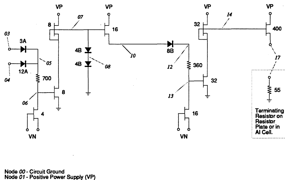
FIGURE 42. FF Cell Circuit Schematic.
