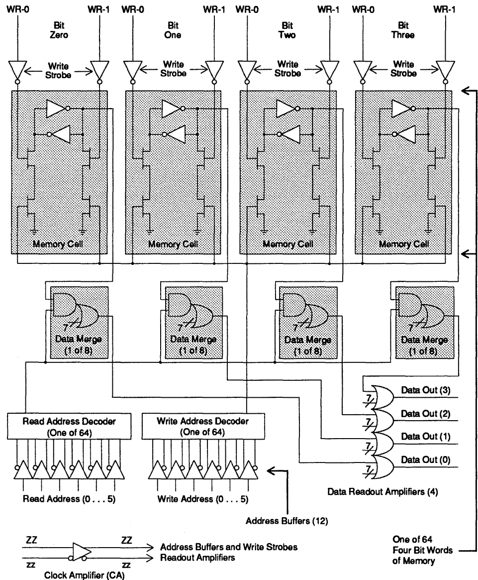
FIGURE 49. Vector Register Block Diagram.
