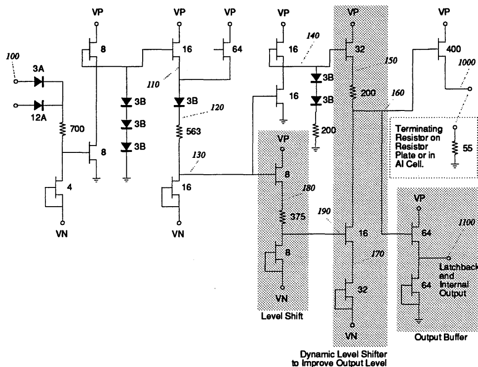
FIGURE 41. FQ Cell Circuit Schematic.
