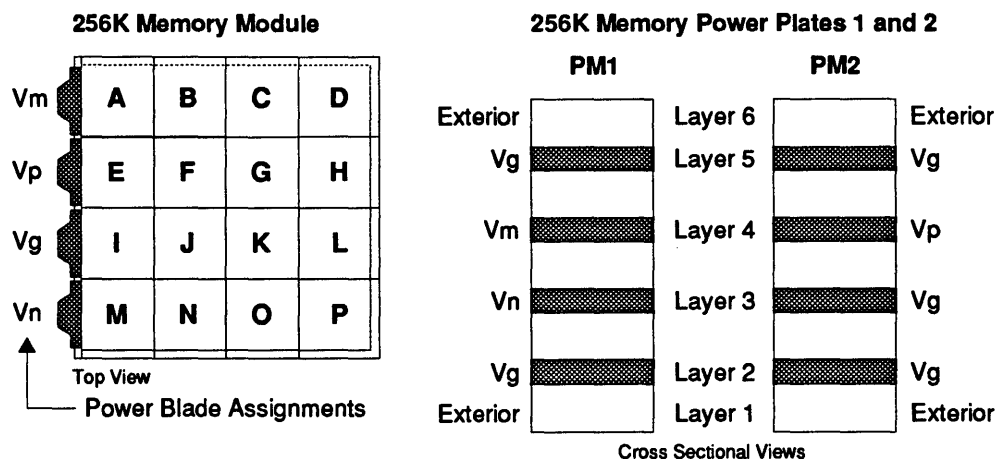
FIGURE 110. Power Distribution in 256K Memory Modules.
