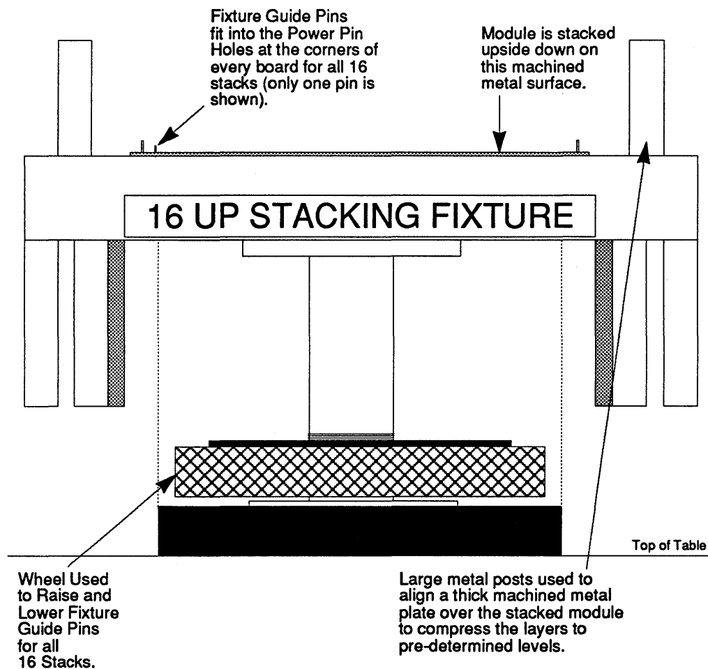
FIGURE 122. Stacking a Module.
