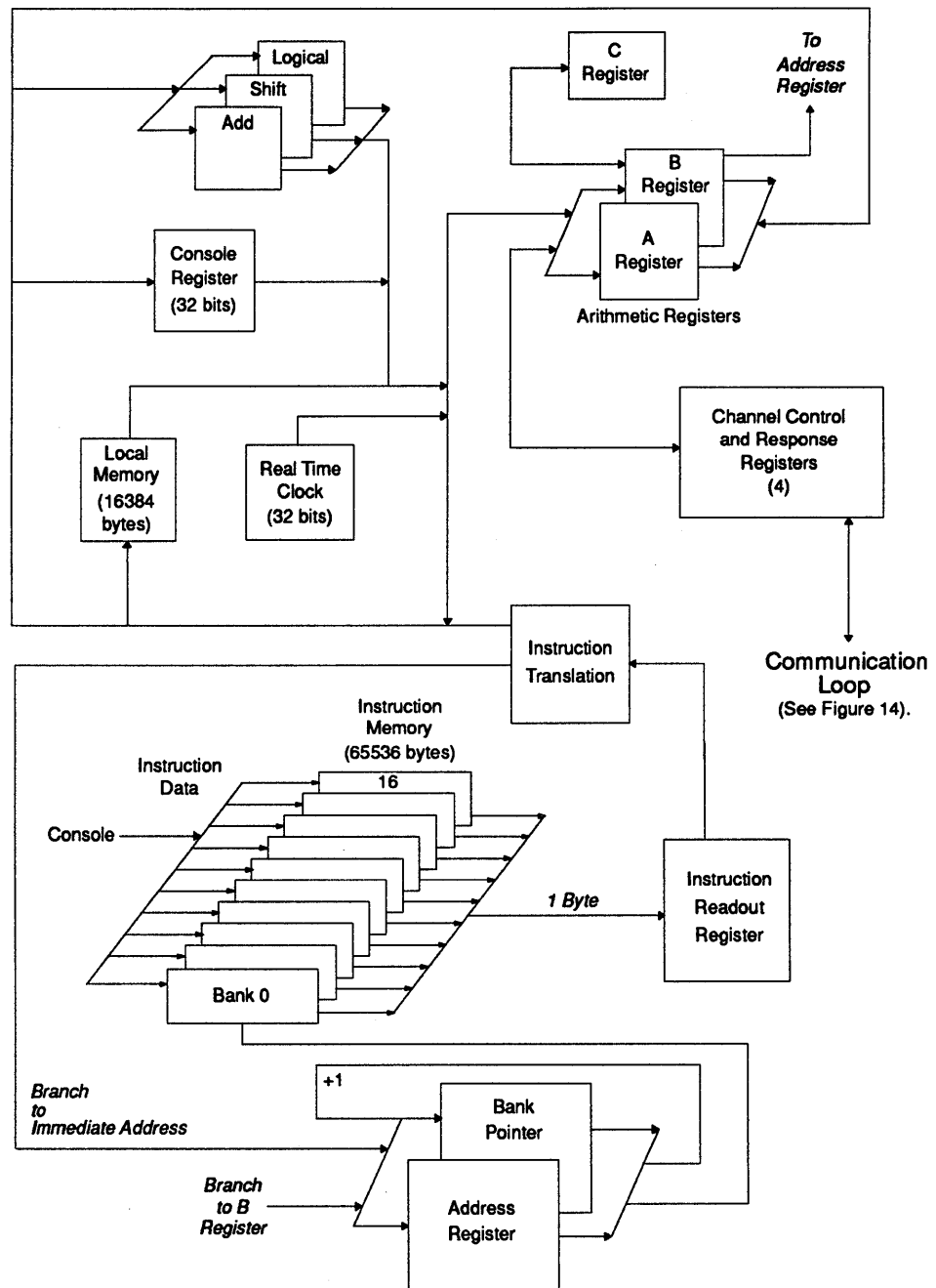
FIGURE 15. Block Diagram of the Foreground Processor.
