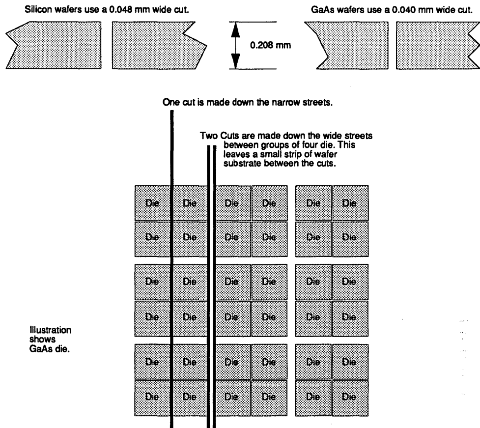
FIGURE 88. Wafer Dicing.
