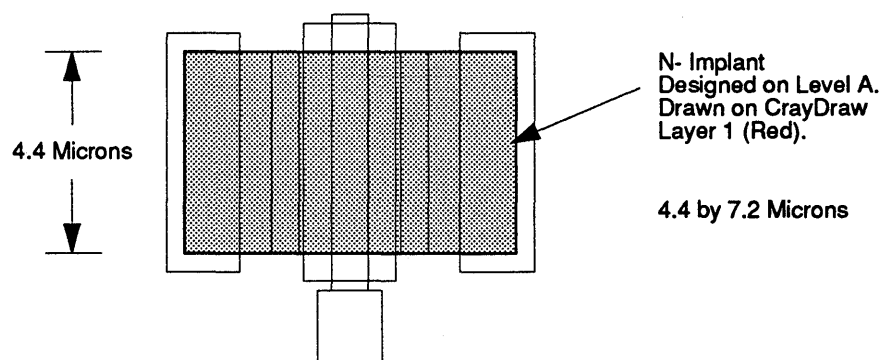
FIGURE 16. 4.0 Micron Transistor—Semiconducting Channel.
