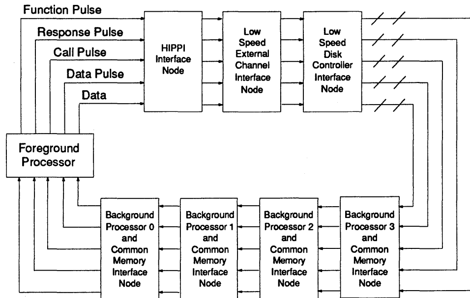
FIGURE 14. Data Channels (One of Four).
