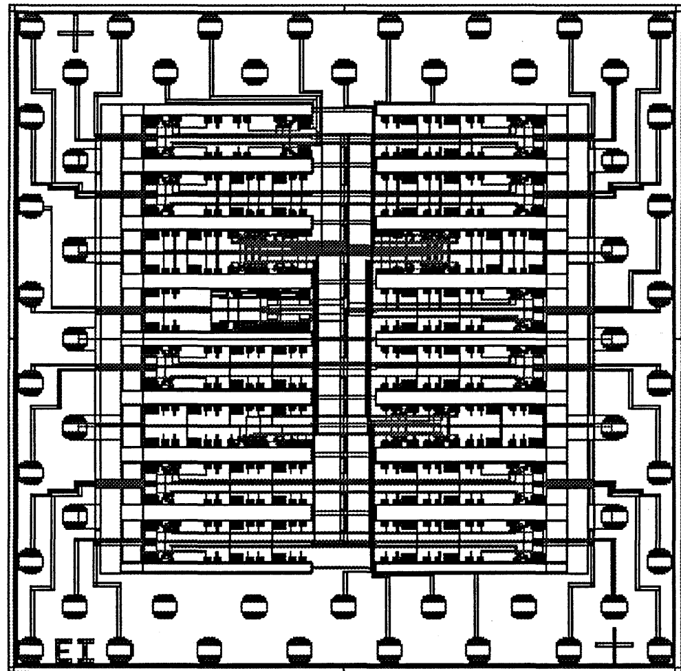
FIGURE 70. Step Three: Routing the Final IC Assembly.
