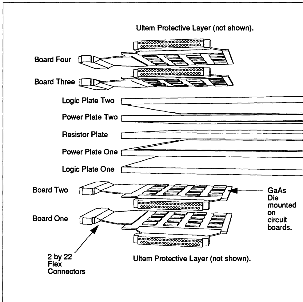
FIGURE 123. Illustration of Stacking Layers.
