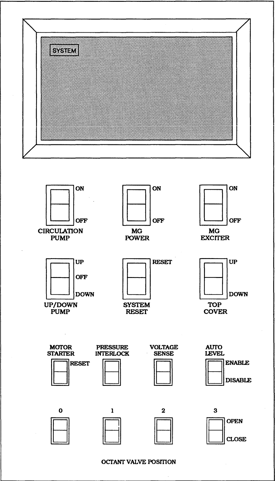
FIGURE 160. C-Pod User Controls.
