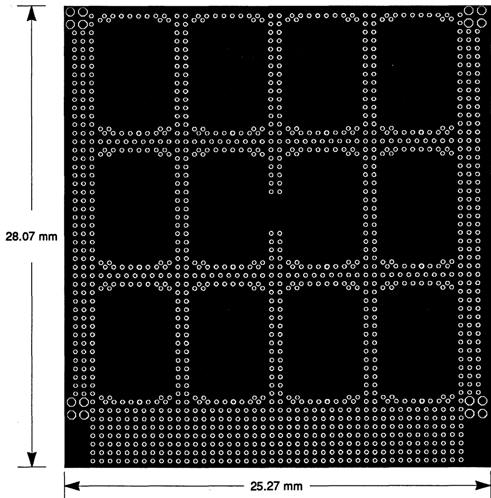
FIGURE 99. 256K Memory Circuit Board.
