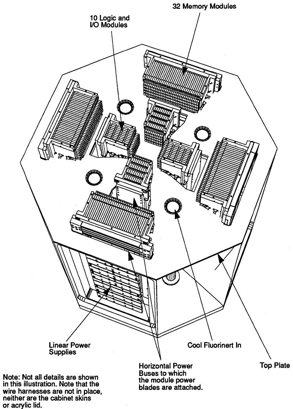
FIGURE 137. Modules Mounted In an Eight-Processor Cabinet.
