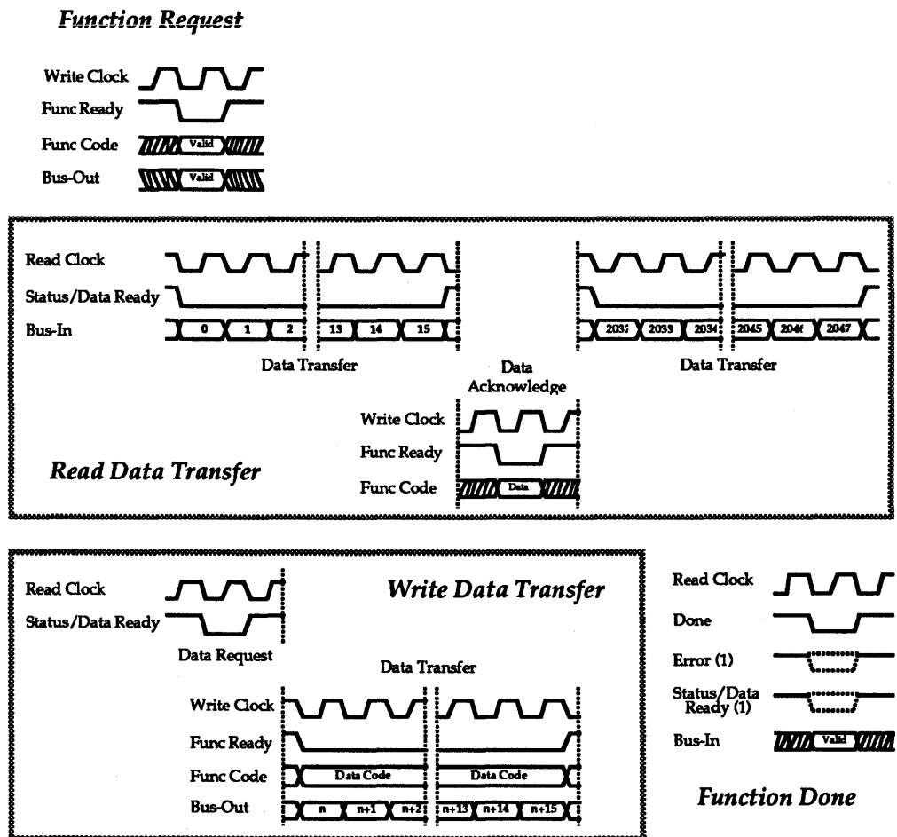
FIGURE 167. Drive Function Timing Sequence.
