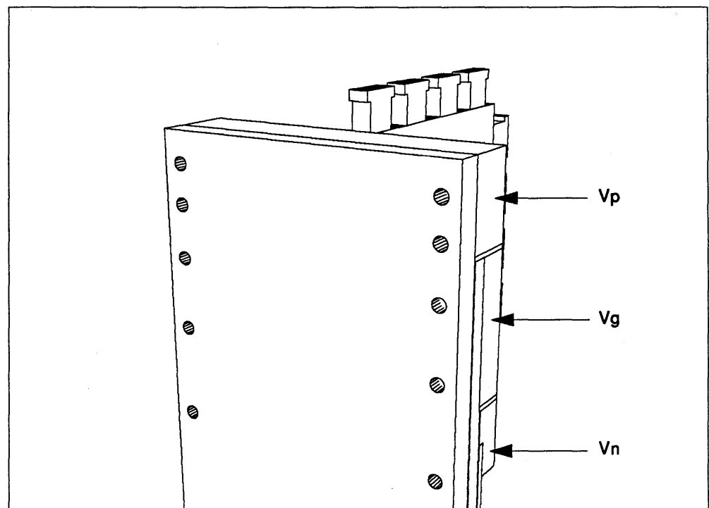
FIGURE 144. Horizontal Power Buses for Logic Modules.
