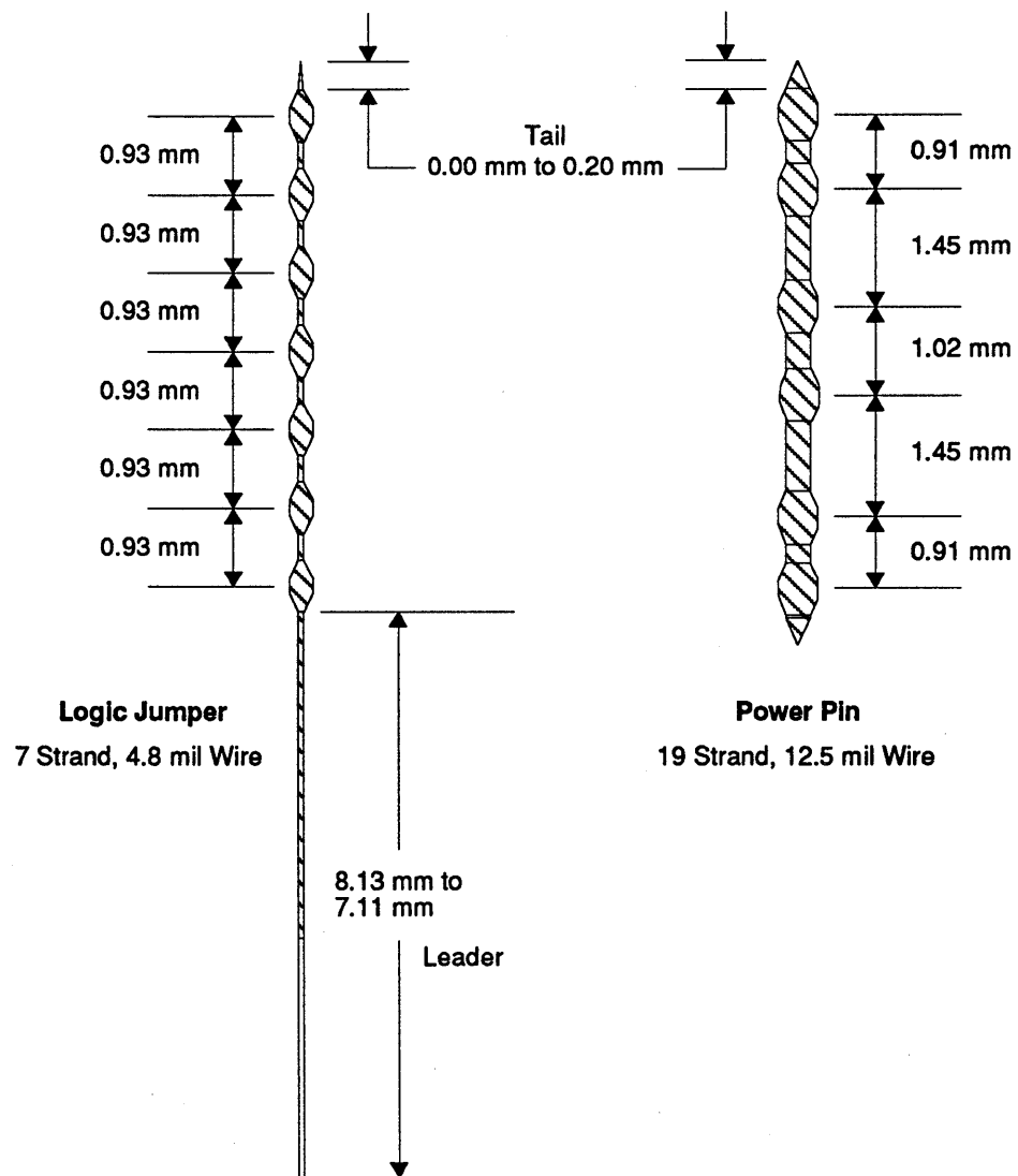
FIGURE 120. Twist Pin Illustrations.
