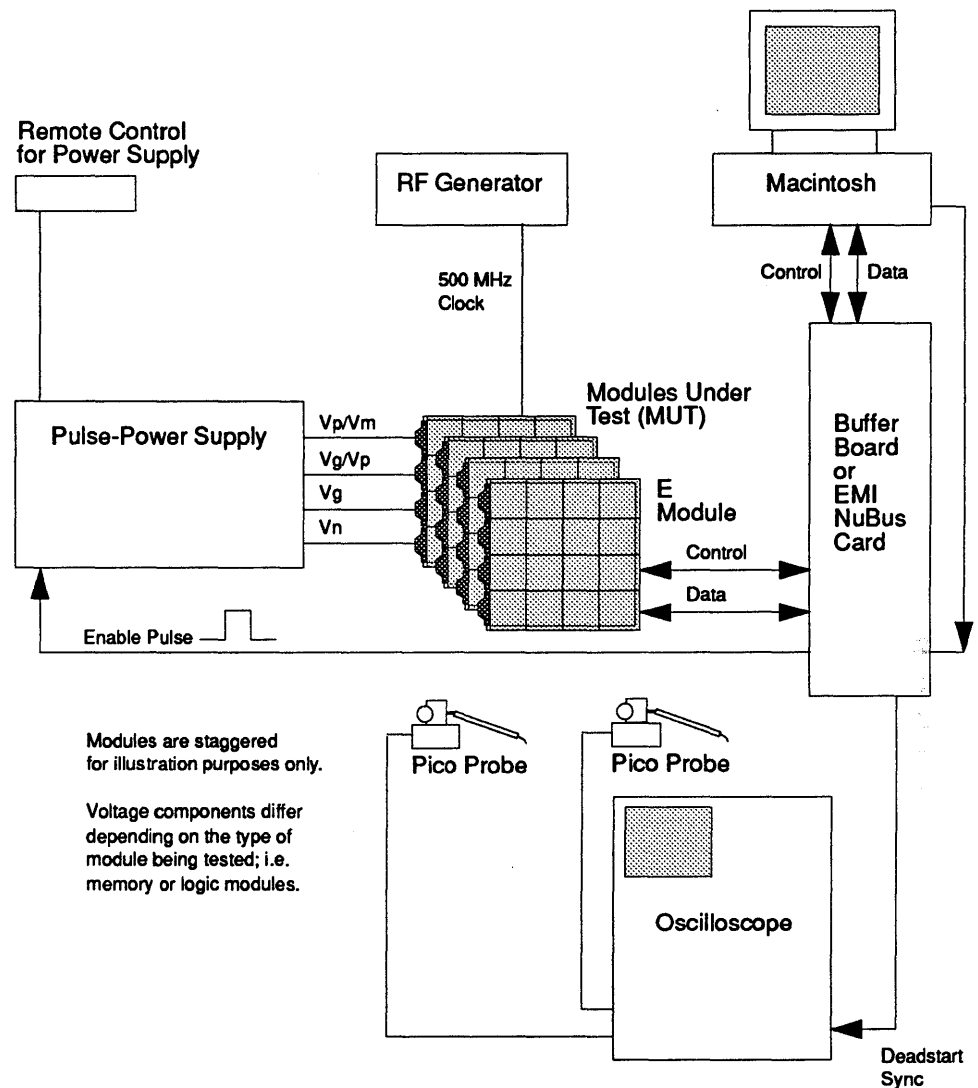
FIGURE 125. Pulse-Power Test Station.
