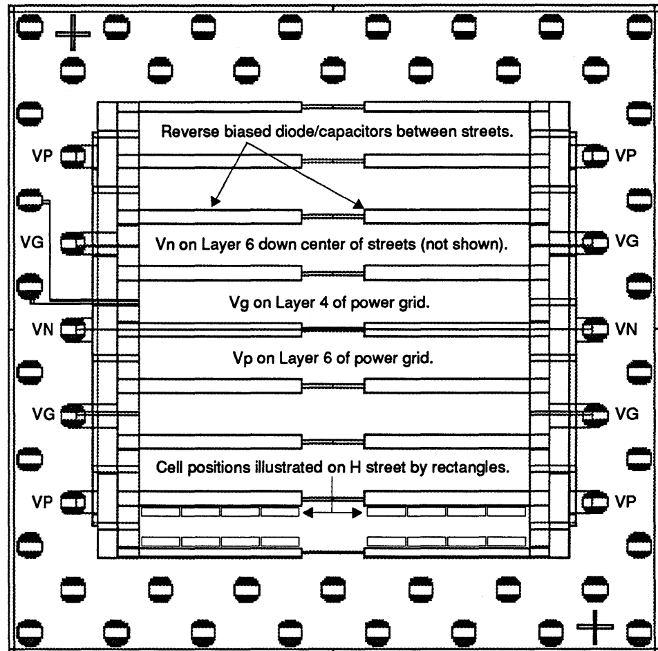
FIGURE 36. Logic Package Power Grid and Cell Positions.
