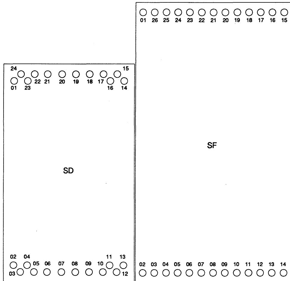
FIGURE 54. SD and SE Die Pinouts.
