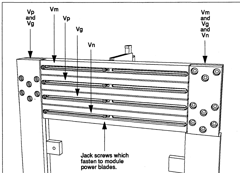
FIGURE 142. Horizontal Power Buses for the Memory Modules.
