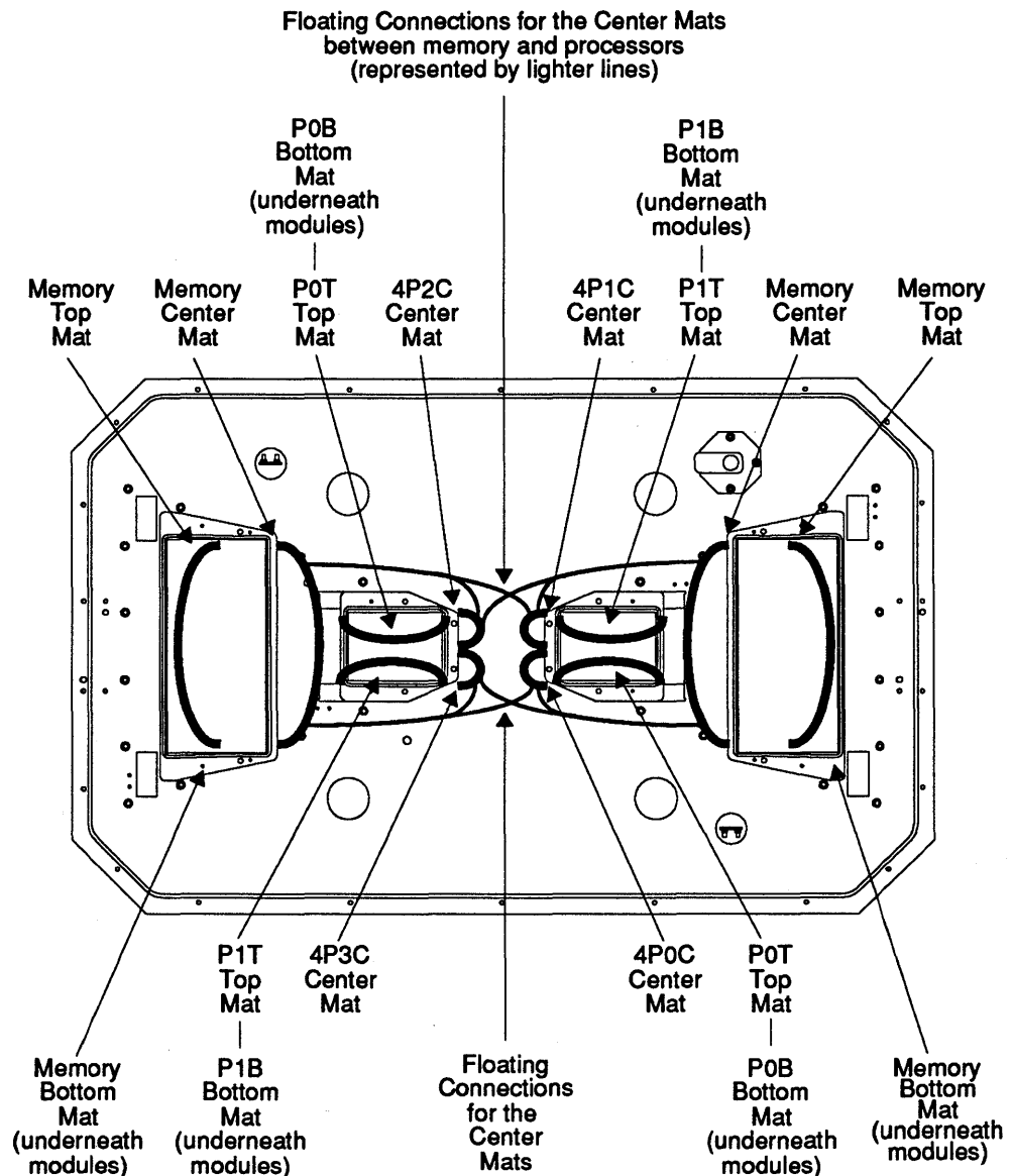
FIGURE 151. Simplified Diagram of Four-Processor Wire Harness.
