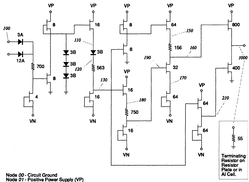
FIGURE 43. FJ Cell Circuit Schematic.
