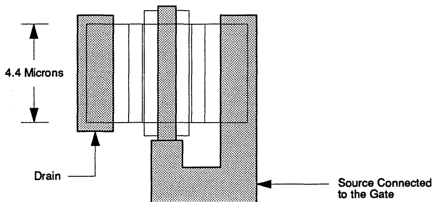
FIGURE 22. 4.0 Micron Current Source—First Layer Metal.
