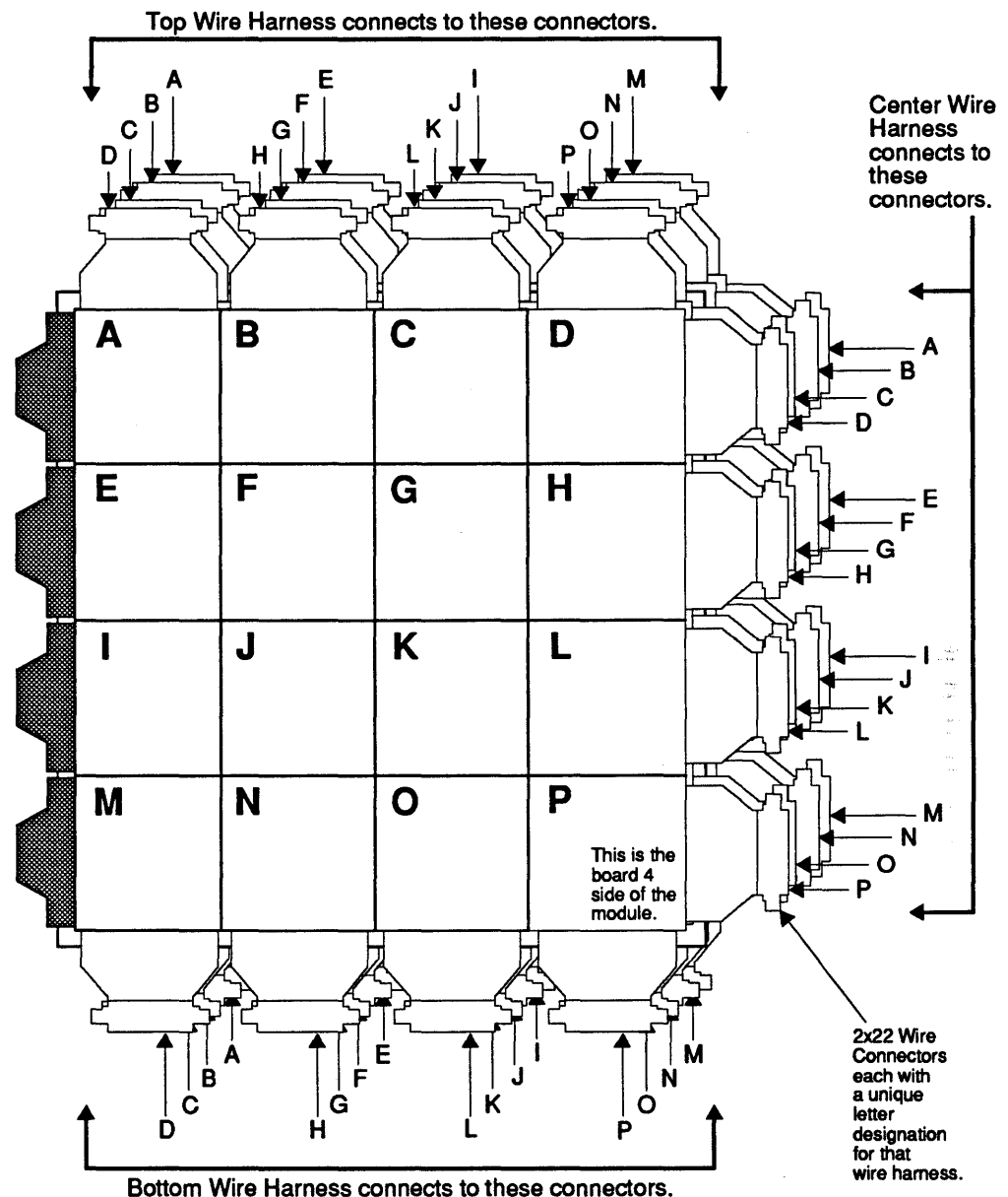
FIGURE 150. Wire Harness Connection Points to the Modules.
