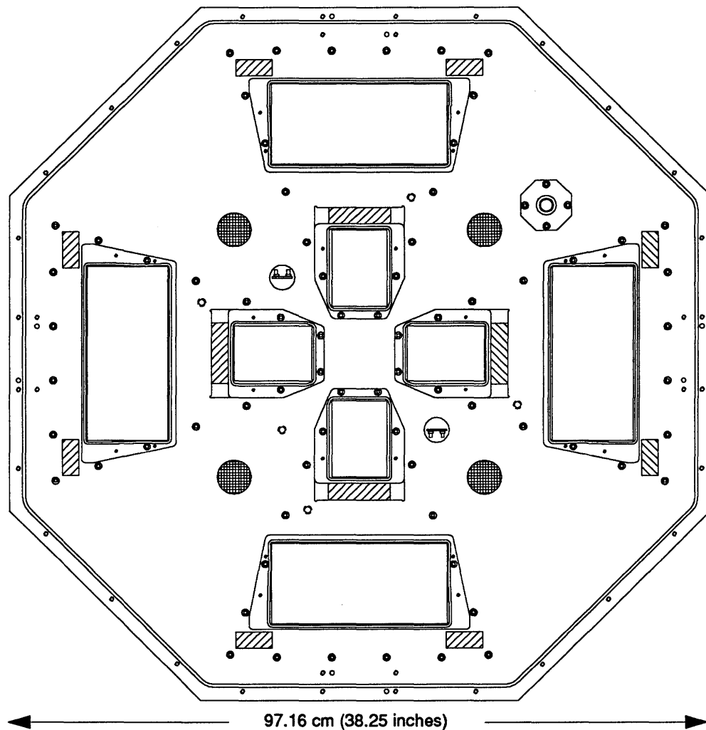
FIGURE 136. Top Plate for an Eight-Processor CRAY-3.
