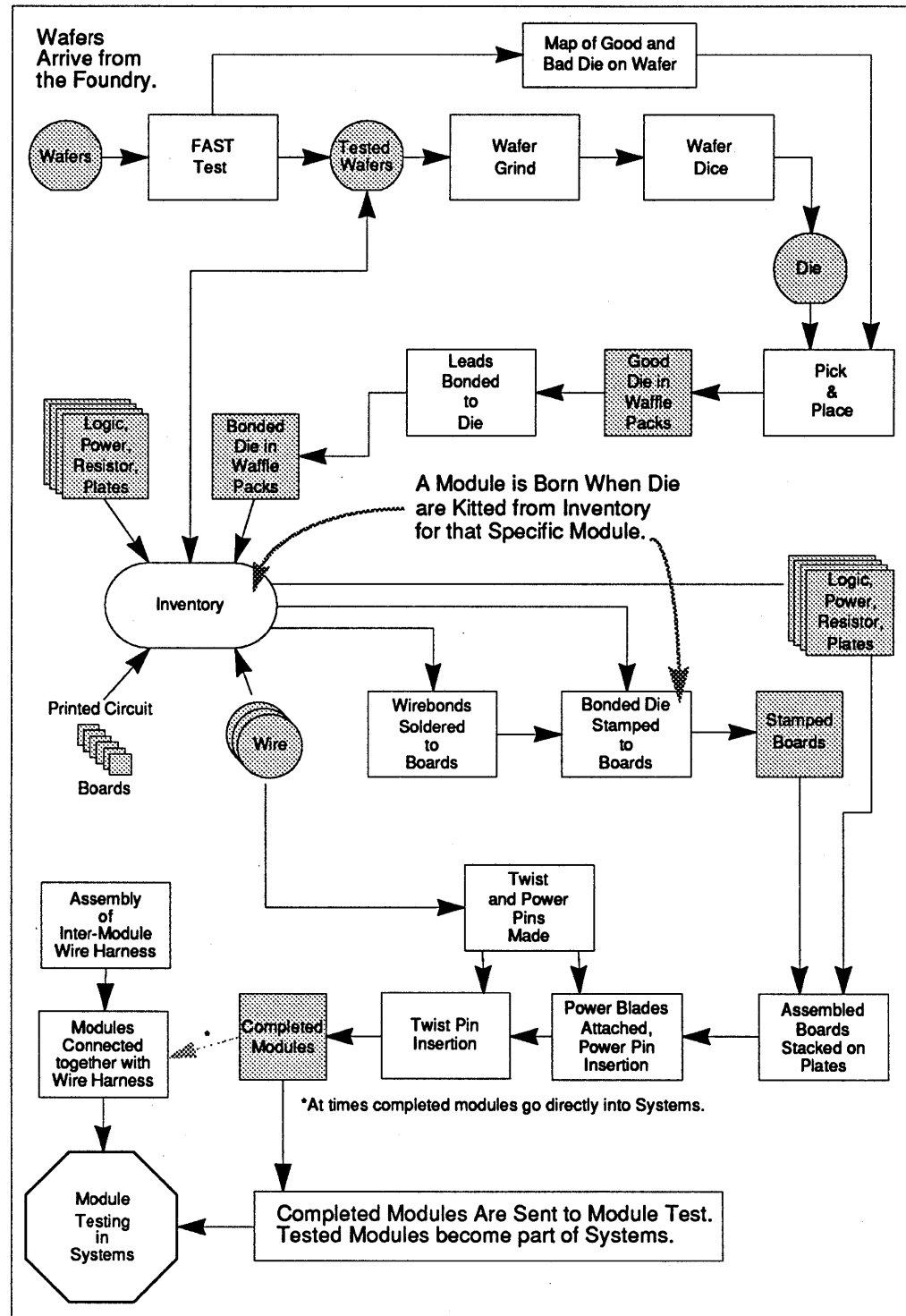
FIGURE 114. Module Build Flow Chart.
