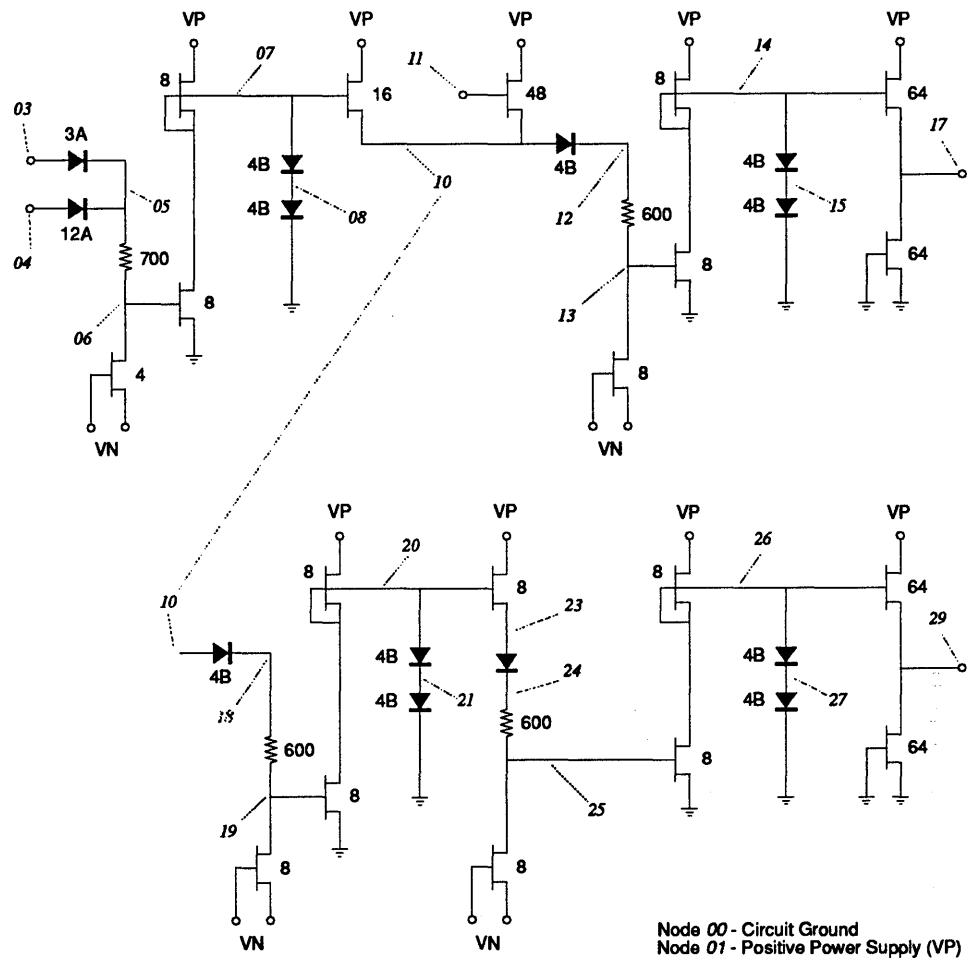
FIGURE 39. ED Cell Circuit Schematic.
