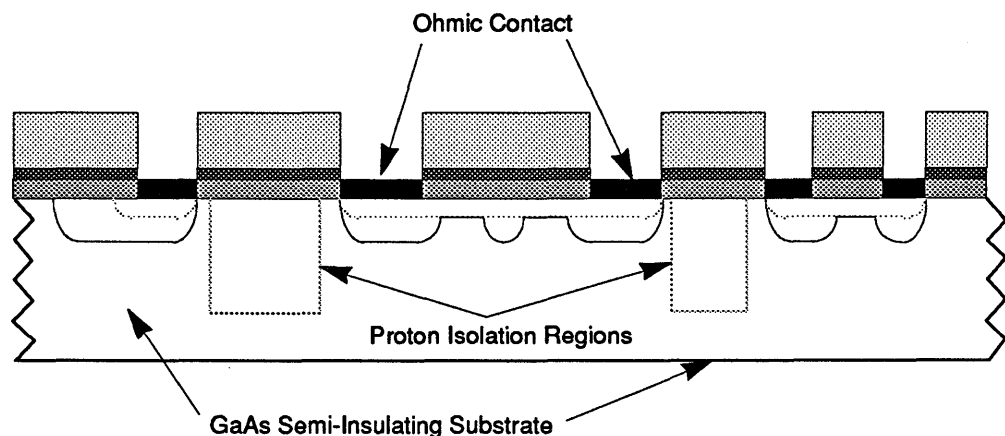
FIGURE 84. Ohmic Contact Metallization and Proton Isolation.
