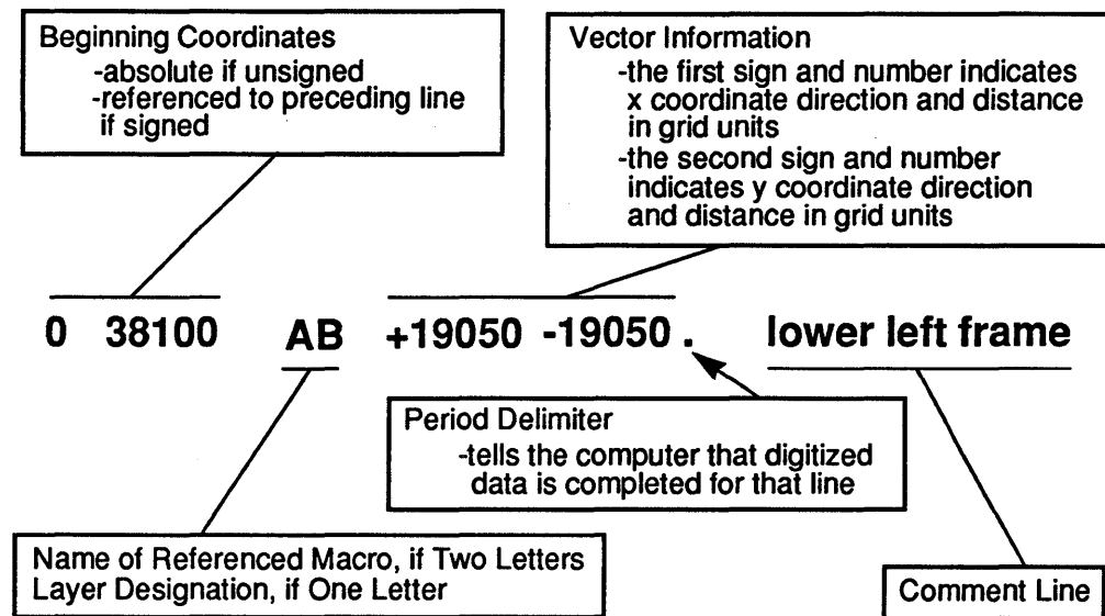
FIGURE 57. Parts of a Macro Text Line.
