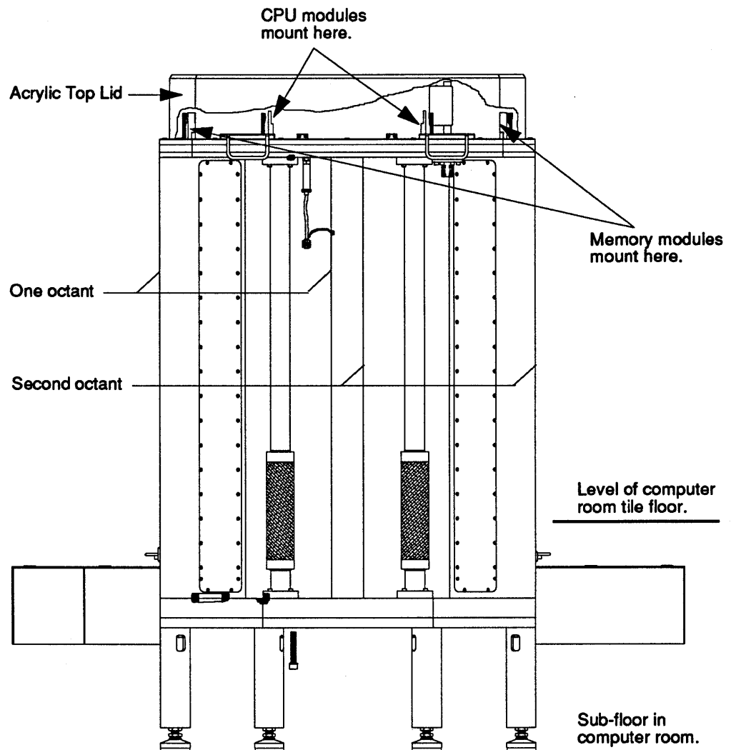
FIGURE 133. Sub-Floor Mounting of the System Cabinet.
