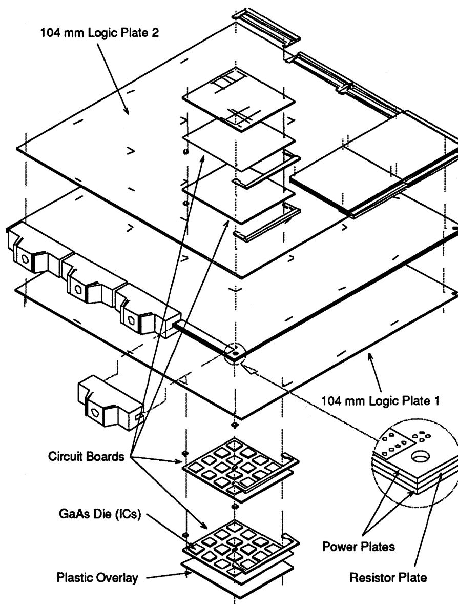
FIGURE 92. Exploded View of a CRAY-3 Module.
