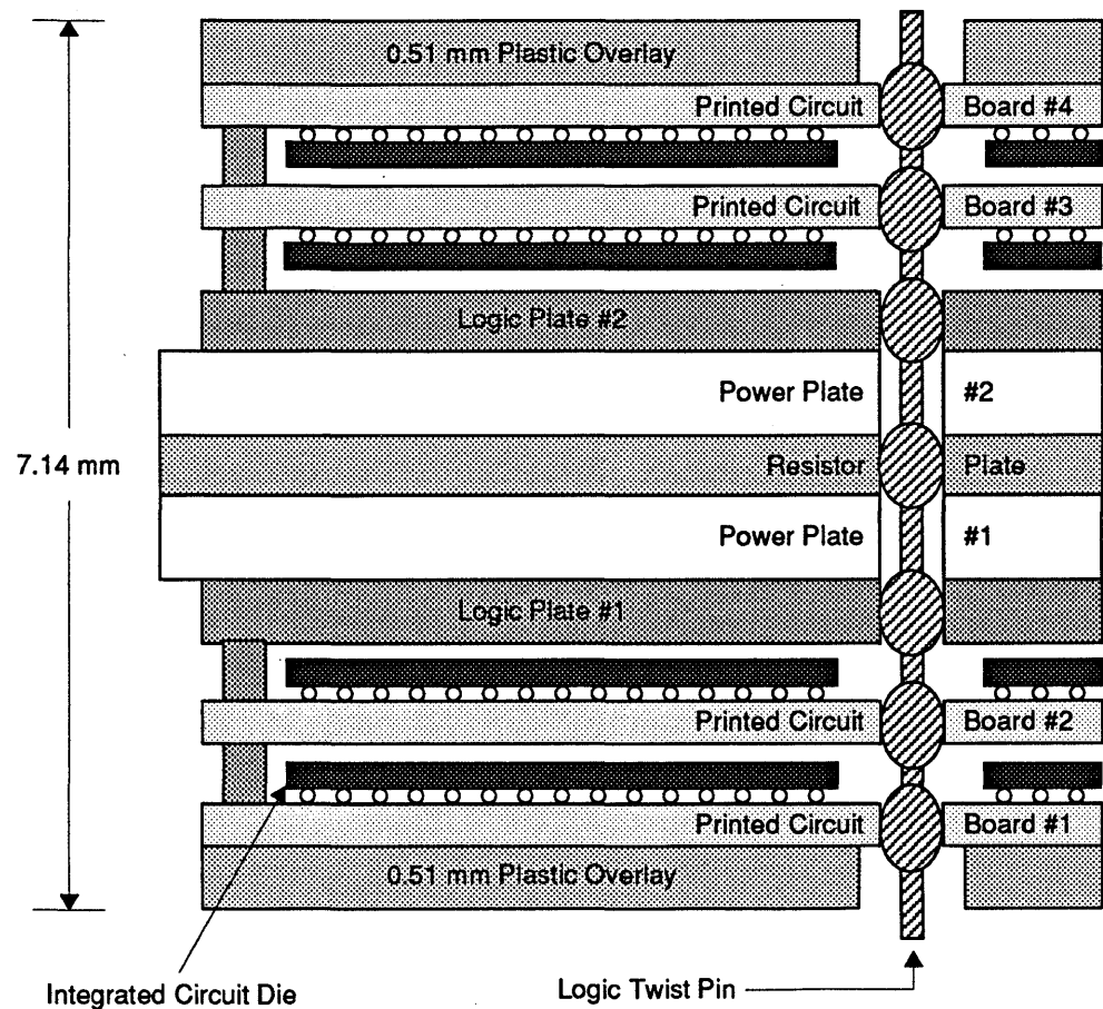
FIGURE 6. Layers in a Module.
