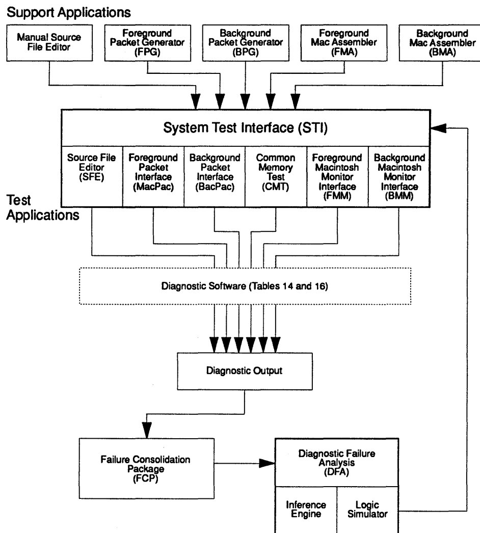
FIGURE 128. Block Diagram of the System Test Interface.
