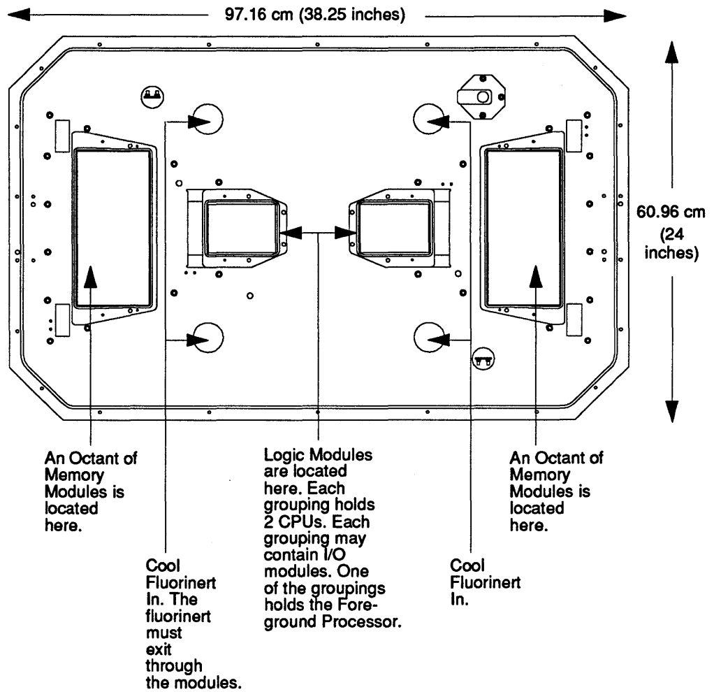
FIGURE 135. Top Plate for a Four-Processor CRAY-3.
