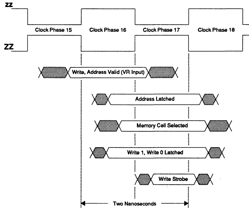
FIGURE 50. VR Write Timing.
