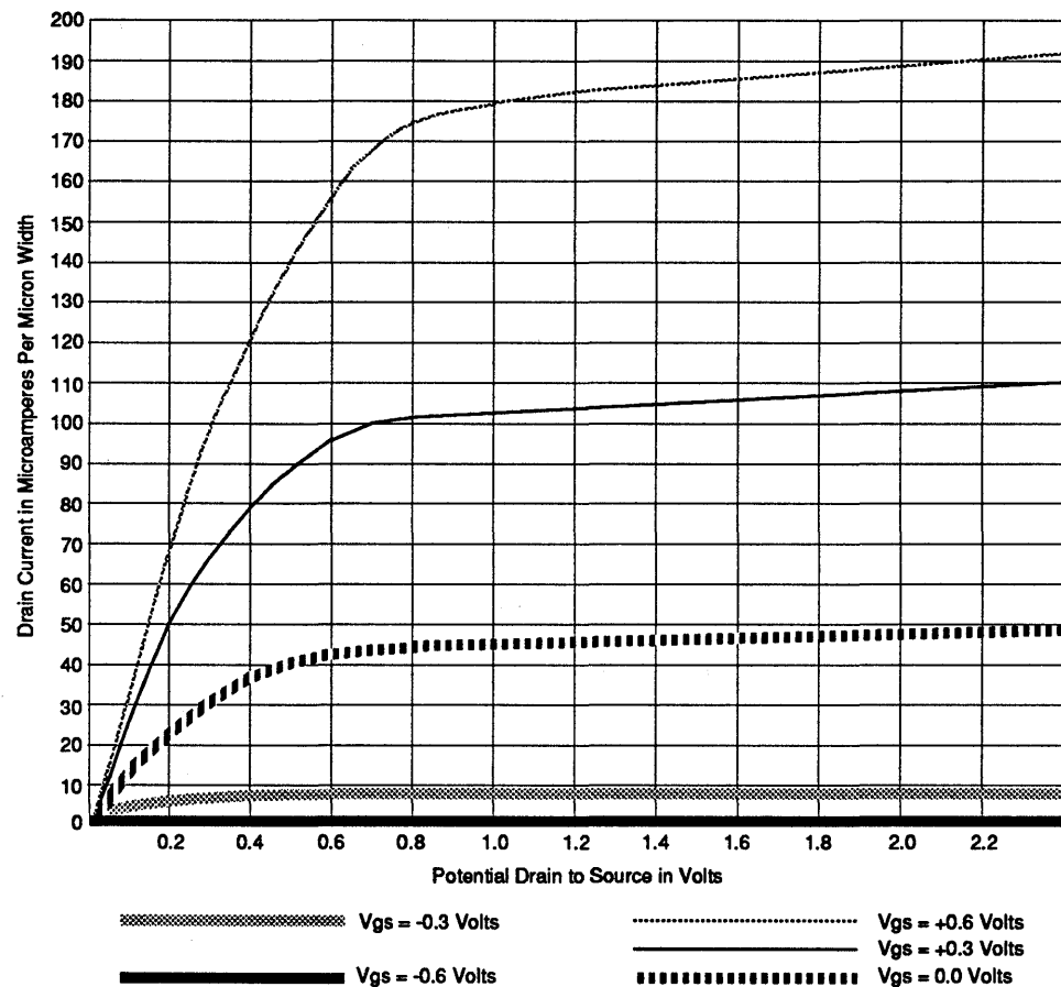
FIGURE 21. Electrical Characteristics of a Transistor.
