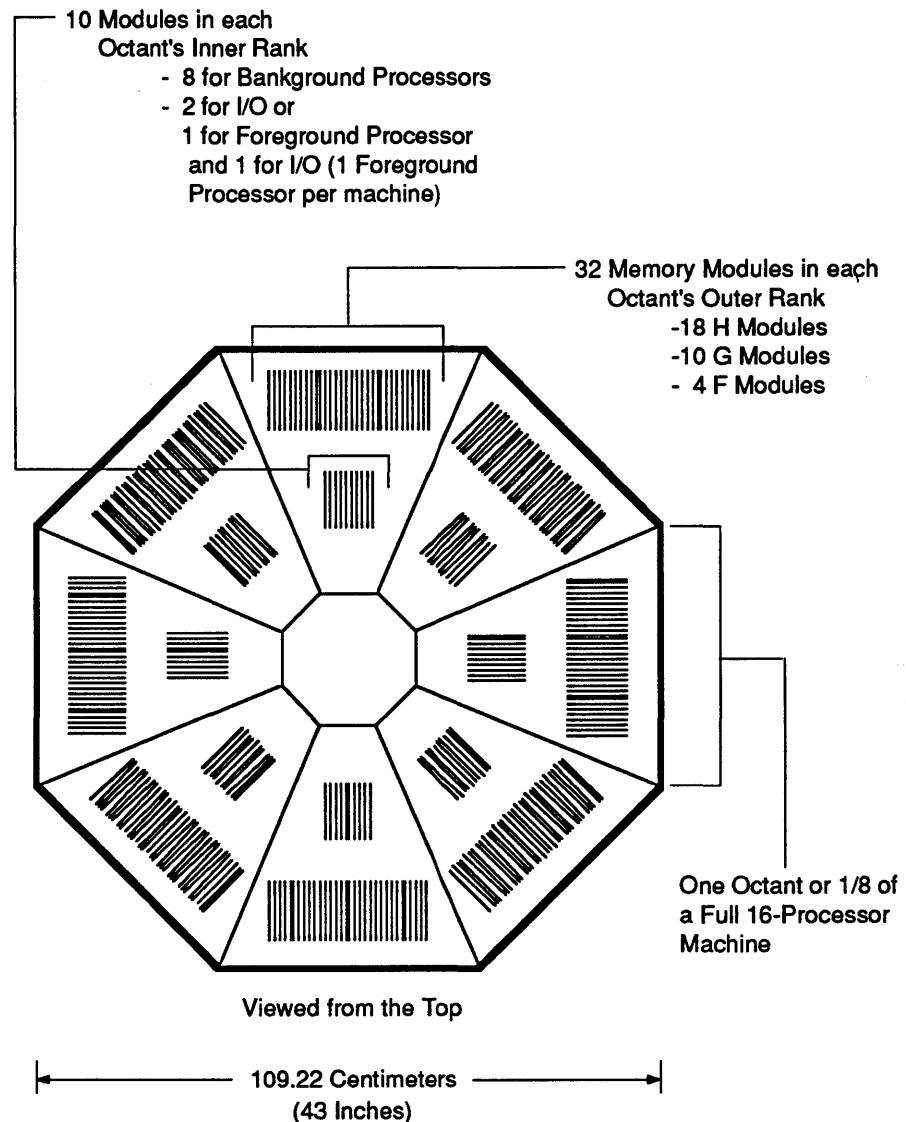
FIGURE 3. Module Placement In the CRAY-3.
