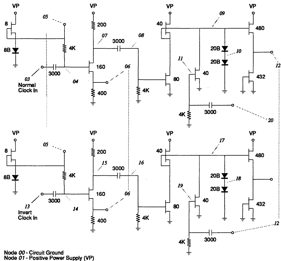
FIGURE 45. CC Cell Circuit Schematic.
