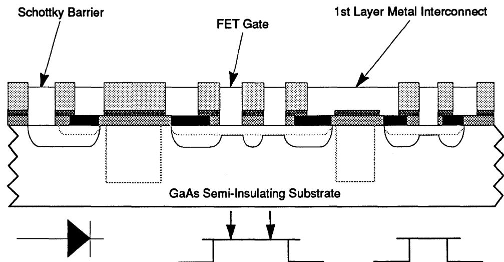
FIGURE 85. Schottky Barrier and First Layer Metal Interconnect.
