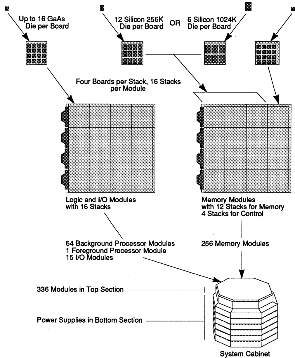
FIGURE 10. Basic Components of the CRAY-3.
