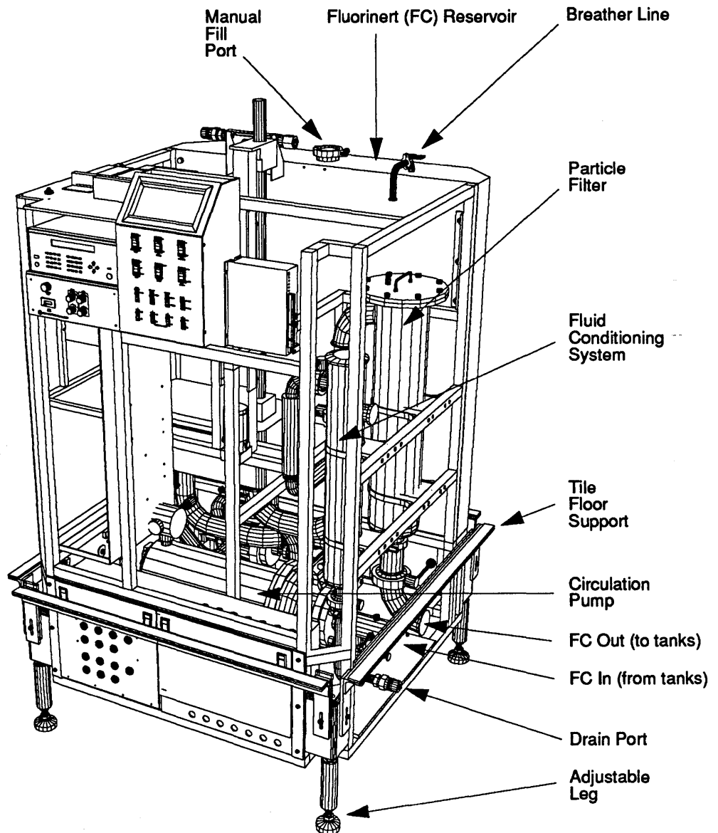
FIGURE 153. C-Pod Cooling Components—Front Right View.
