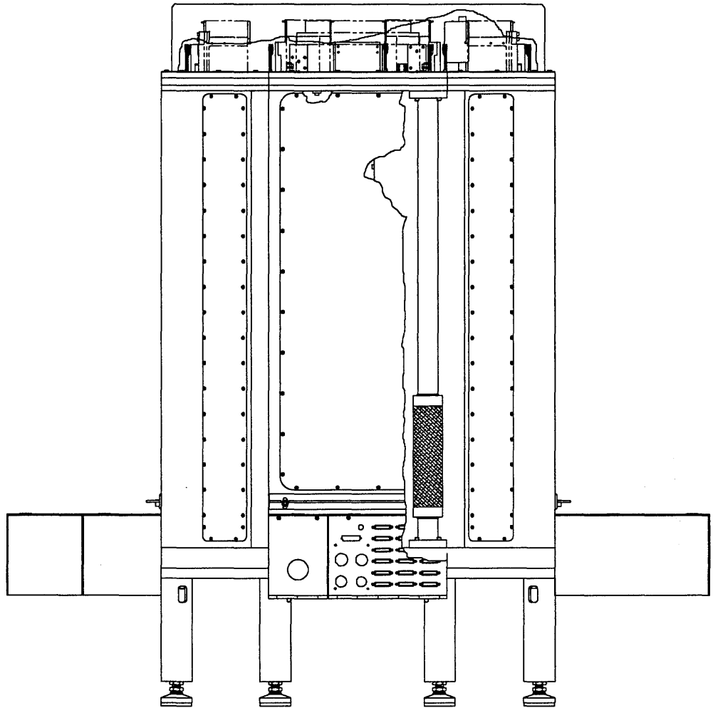
FIGURE 130. Front View of Eight-Processor System Cabinet.
