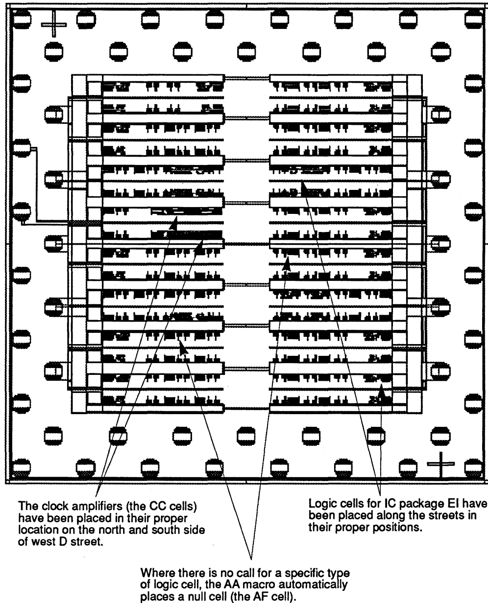
FIGURE 66. Step Two: Placing the Required Logic Cells.
