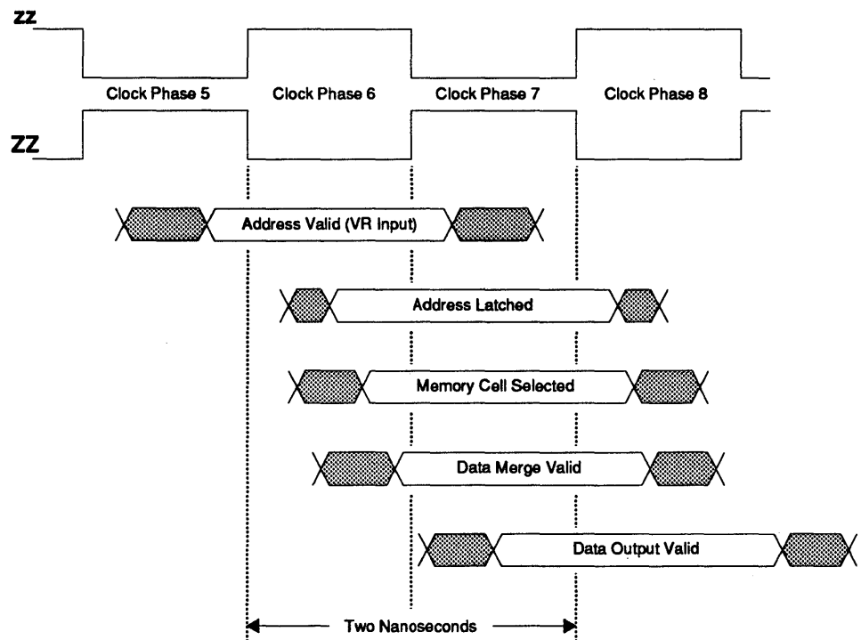
FIGURE 51. VR Read Timing.
