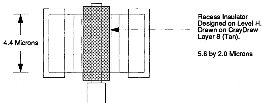
FIGURE 20. 4.0 Micron Transistor—Recess Opening.
