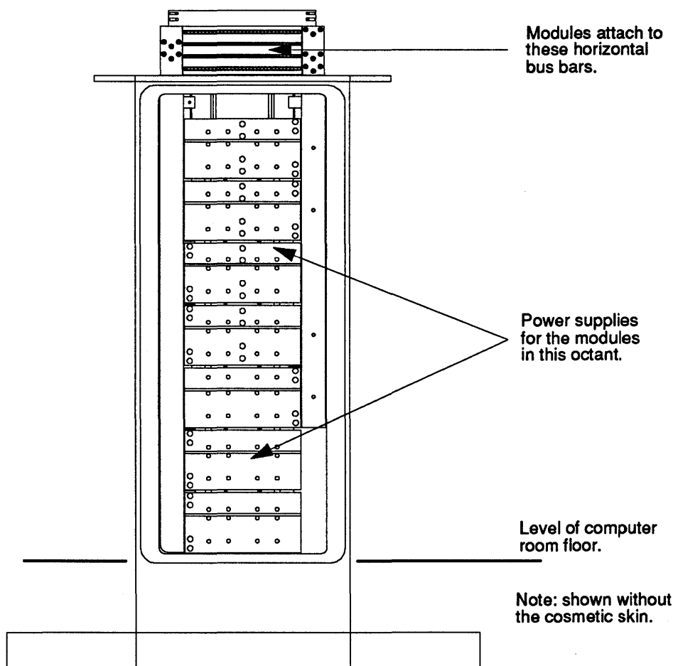
FIGURE 129. Front View of a Four-Processor Tank.
