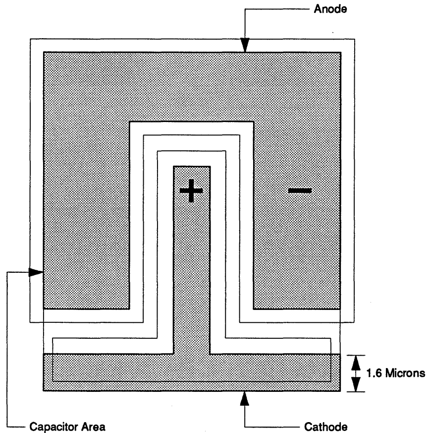
Level D: First Layer Metal.
