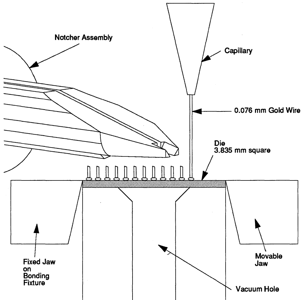
FIGURE 90. Die Bonding Illustration.
