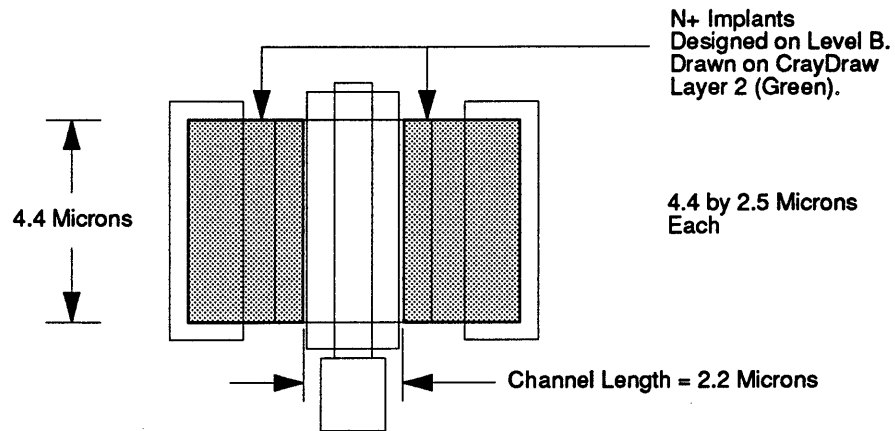
FIGURE 17. 4.0 Micron Transistor—N+ Implants.
