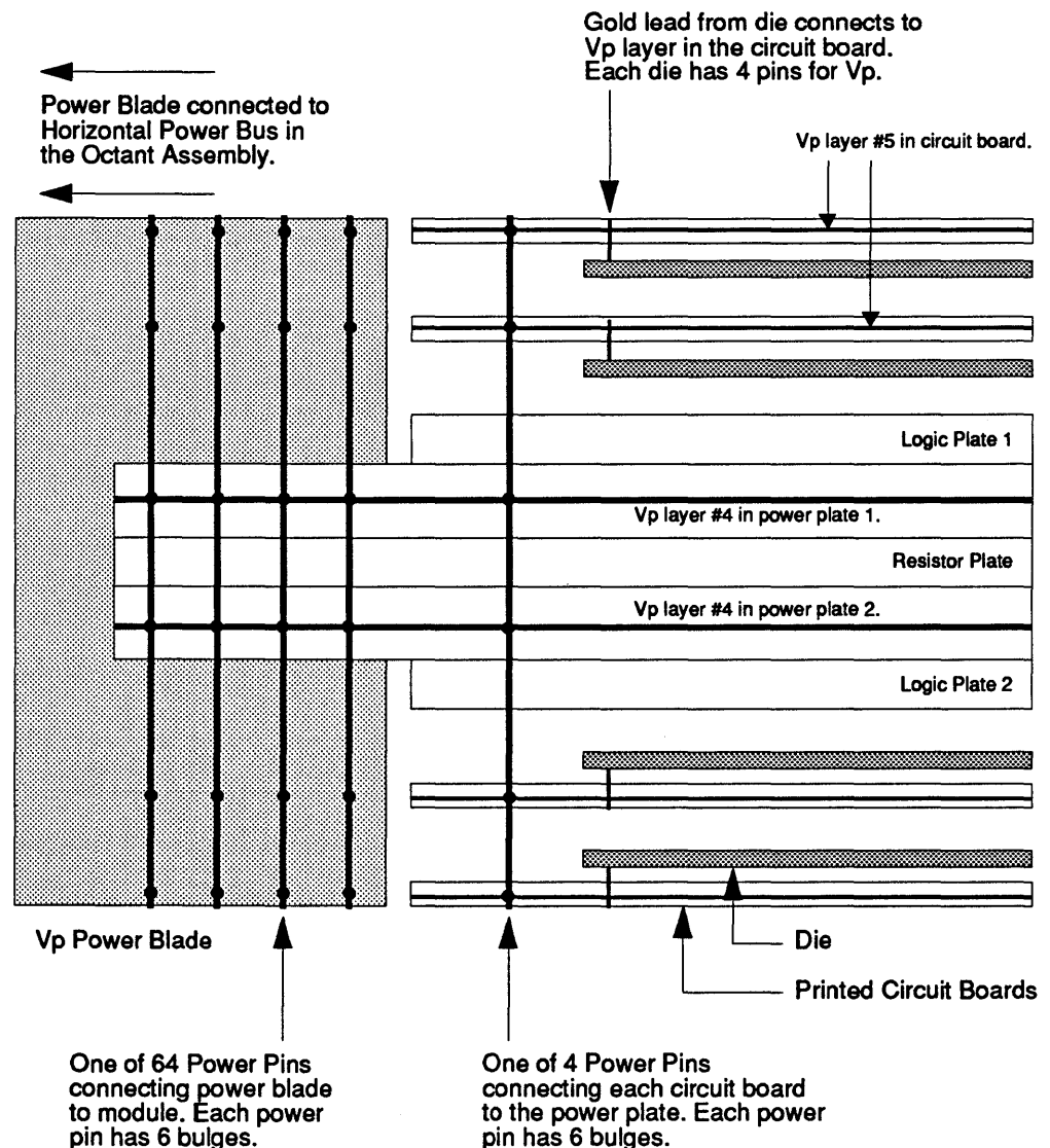
FIGURE 108. Vp Power Distribution In a Module.
