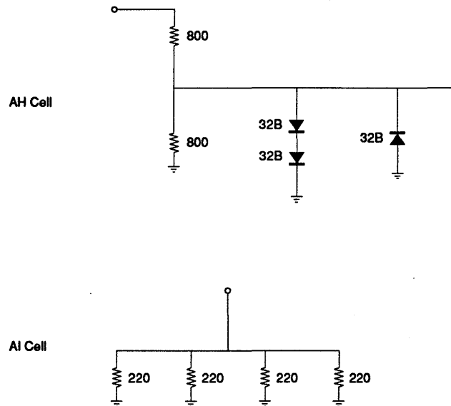
FIGURE 48. AH Cell and AI Cell Circuit Schematics.
