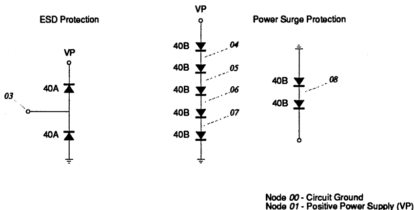
FIGURE 46. AF Cell Circuit Schematic.
