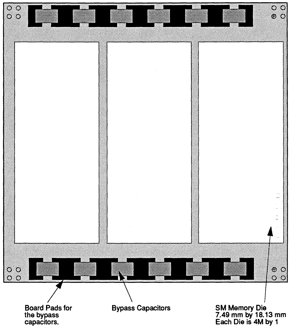
FIGURE 106. SM Die and Bypass Capacitors.
