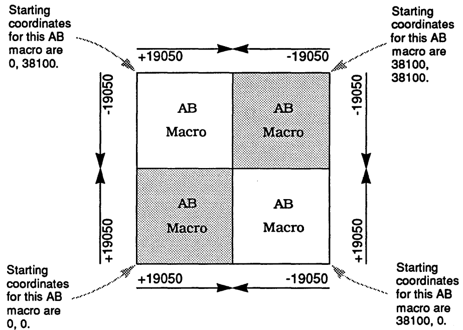
FIGURE 60. Placement of the AB Macro.
