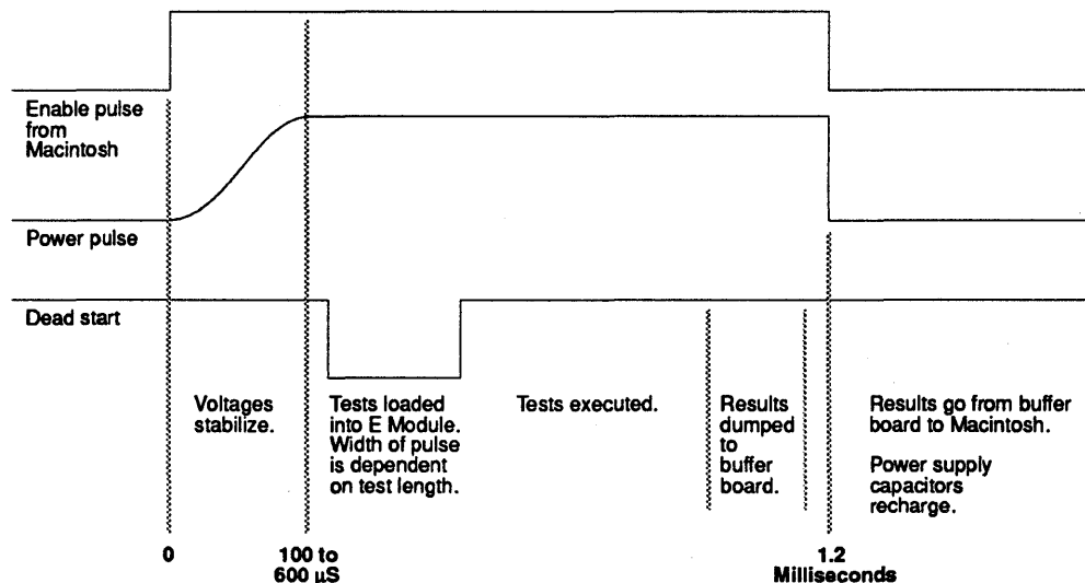
FIGURE 127. Time Chart for Pulse-Power Testing.
