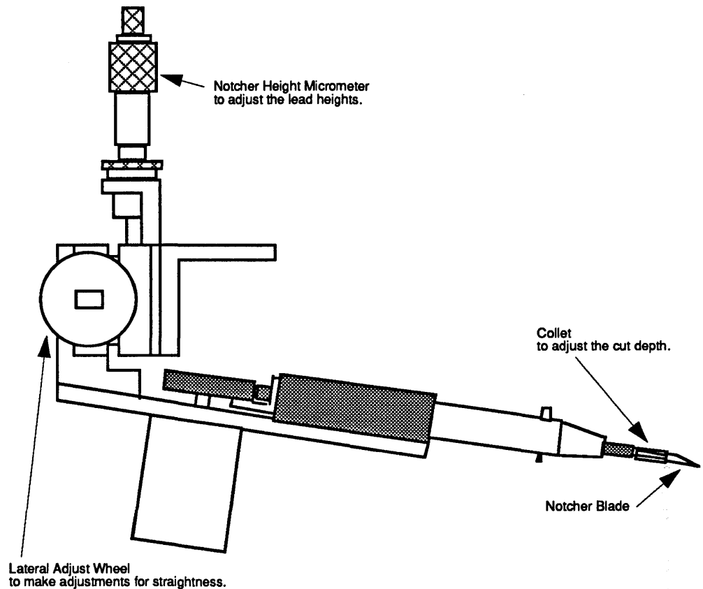
FIGURE 89. Notcher Mechanism.
