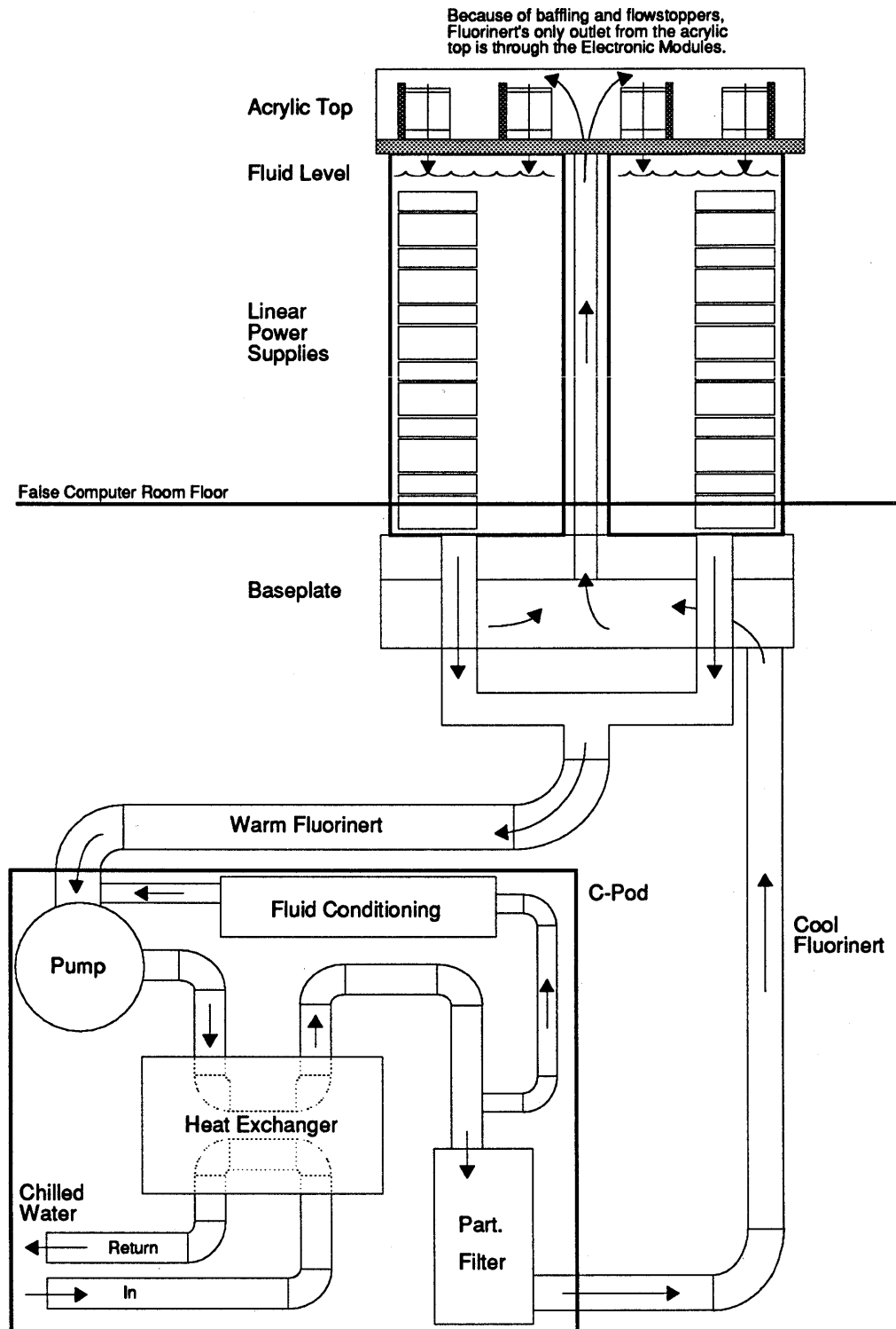
FIGURE 152. Simplified Diagram of the Cooling System.
