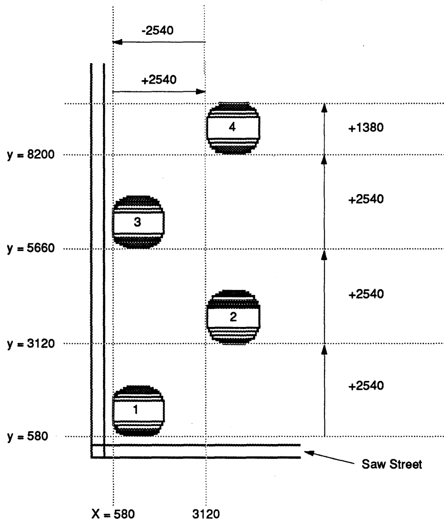
FIGURE 62. Placement of the AC Macros.
