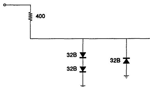
FIGURE 47. AG Cell Circuit Schematic.
