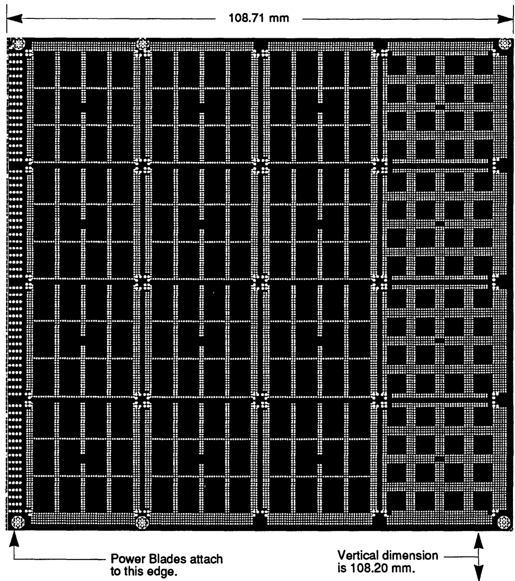
FIGURE 105. 256K Memory Module Power Plate.
