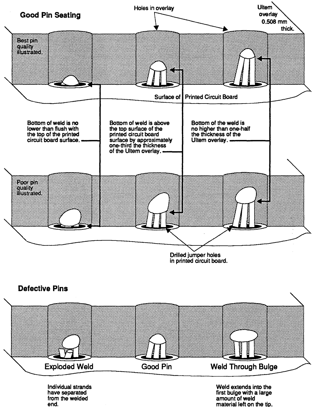
FIGURE 124. Twist Pin Seating.
