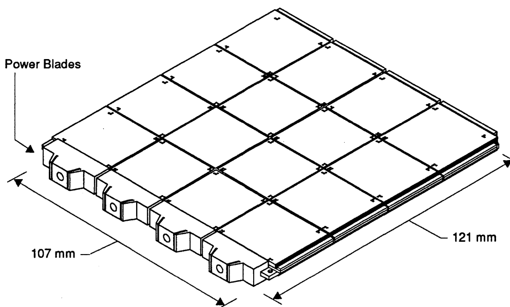
FIGURE 5. CRAY-3 Electronic Module.
