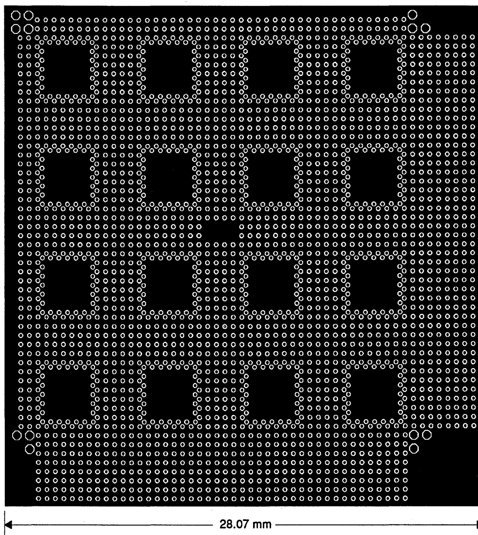
FIGURE 97. P Stack Logic Circuit Board.
