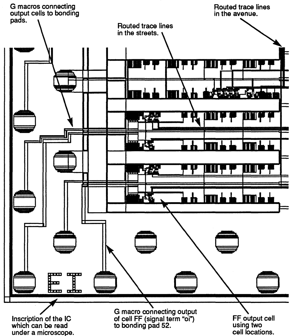
FIGURE 71. Bottom Left Corner of the EI Package.
