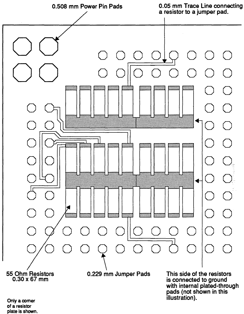
FIGURE 104. Resistors on a Logic Module Resistor Plate.
