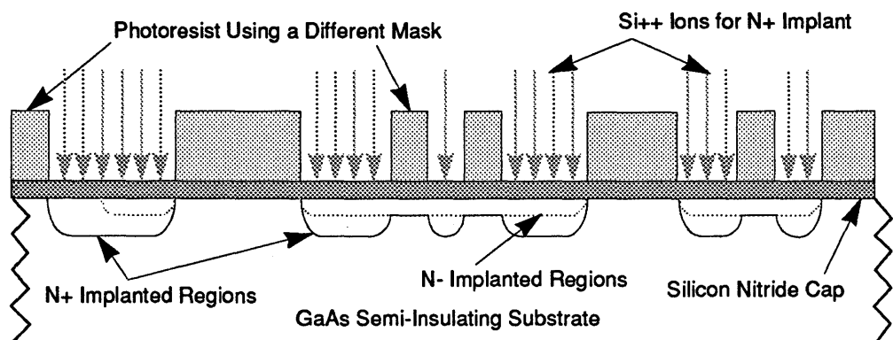
FIGURE 83. Heavy Ion (N+) Implant.
