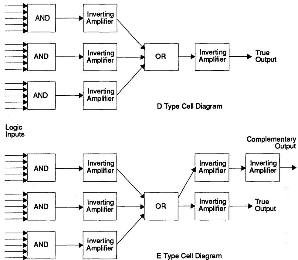
FIGURE 35. Logic Package Block Diagrams.
