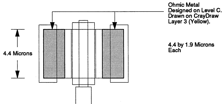
FIGURE 18. 4.0 Micron Transistor—Ohmic Metal.
