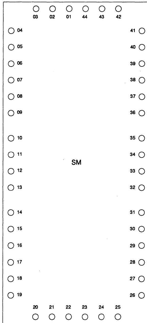
FIGURE 55. SM Die Pinouts.
