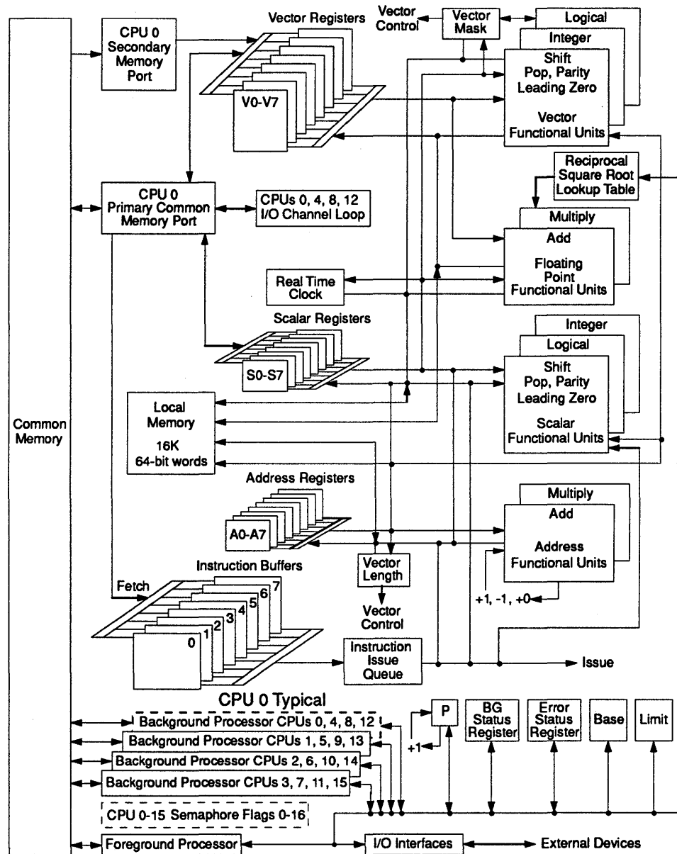
FIGURE 12. Block Diagram of a Background Processor.
