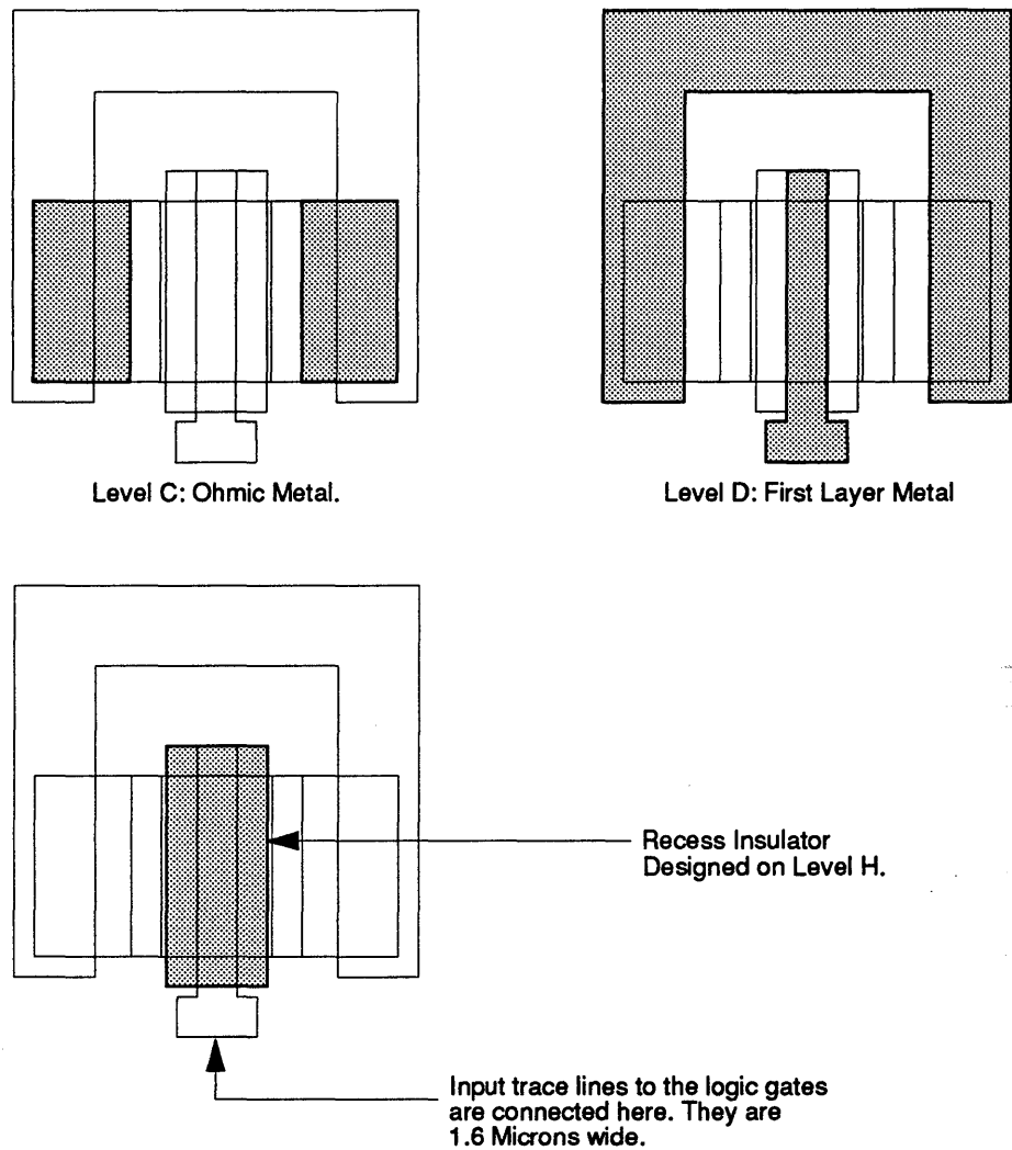
FIGURE 24. Type A Diode—Metal Layers and Recess Insulator.
