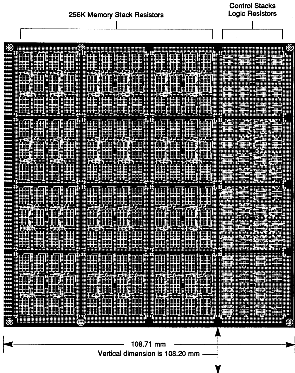
FIGURE 103. 256 K Memory Resistor Plate.
