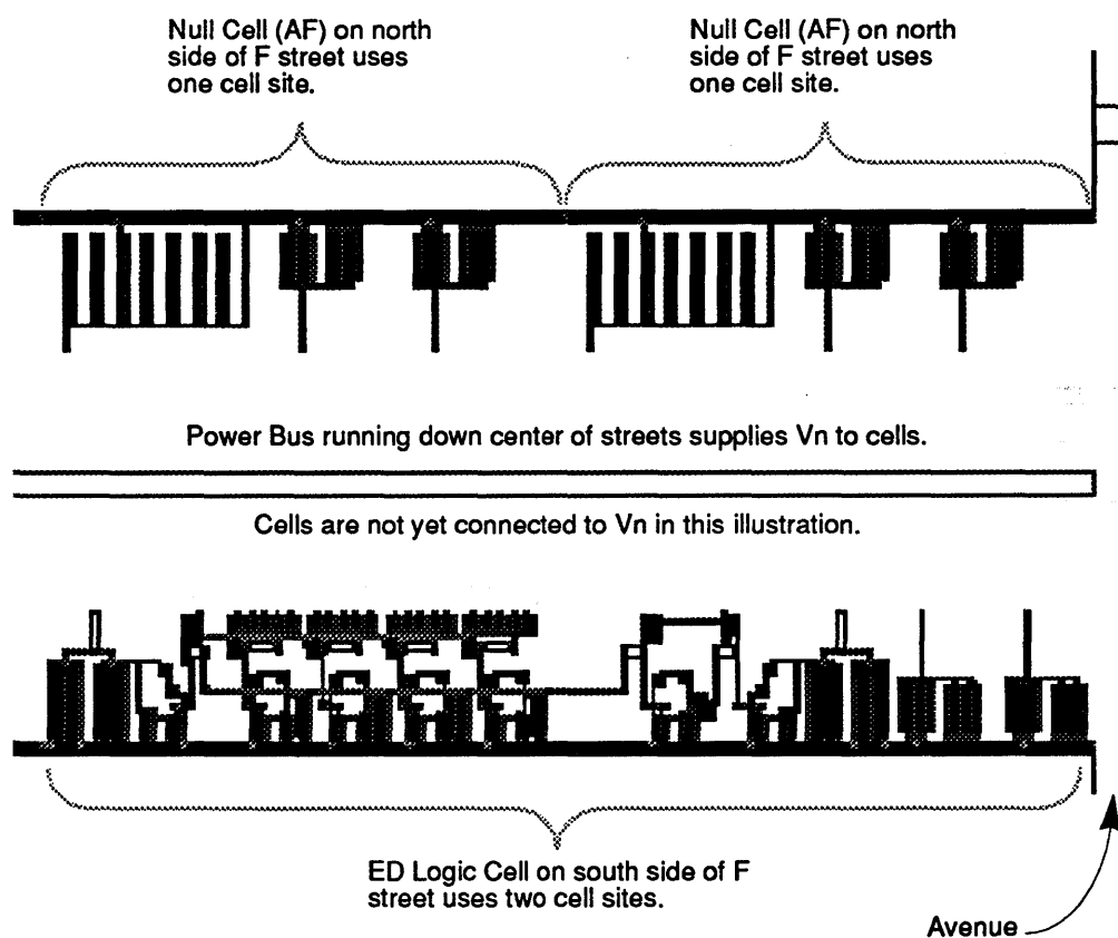
FIGURE 69. Close-Up of Cells on West F Street.
