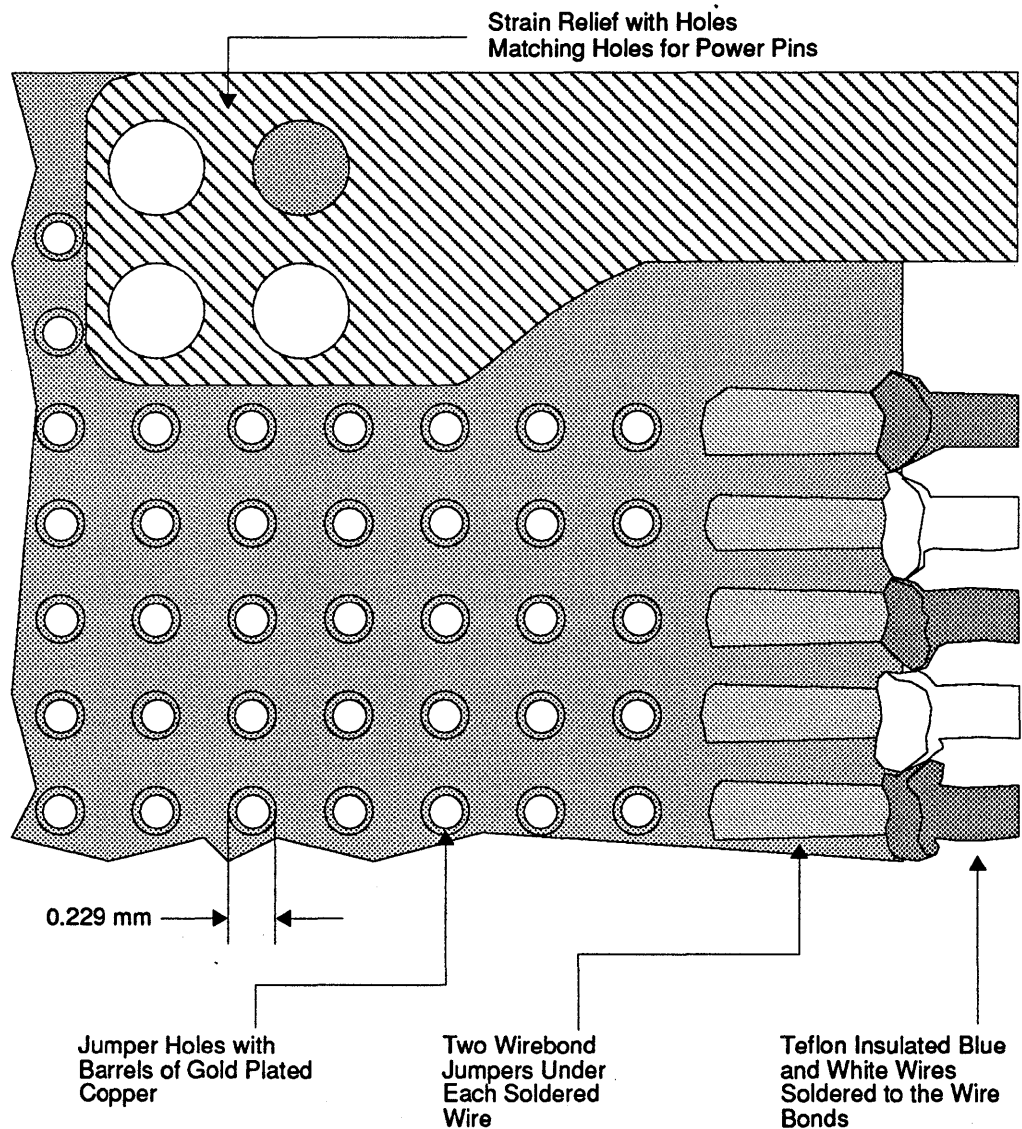
FIGURE 116. Small Wires Soldered to Circuit Boards.
